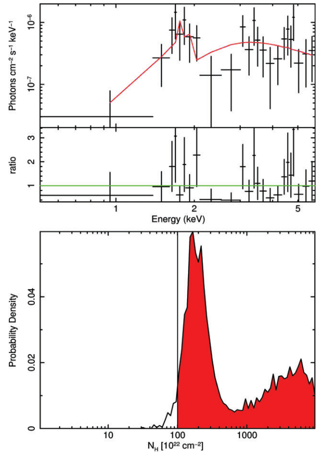
FIGURE 2 (a) Unfolded spectrum and data/model ratio of the CT candidate LID_1002 at z = 2.612 . This source required only the BNtorus component. (b) PDF of N_H for the same source.
