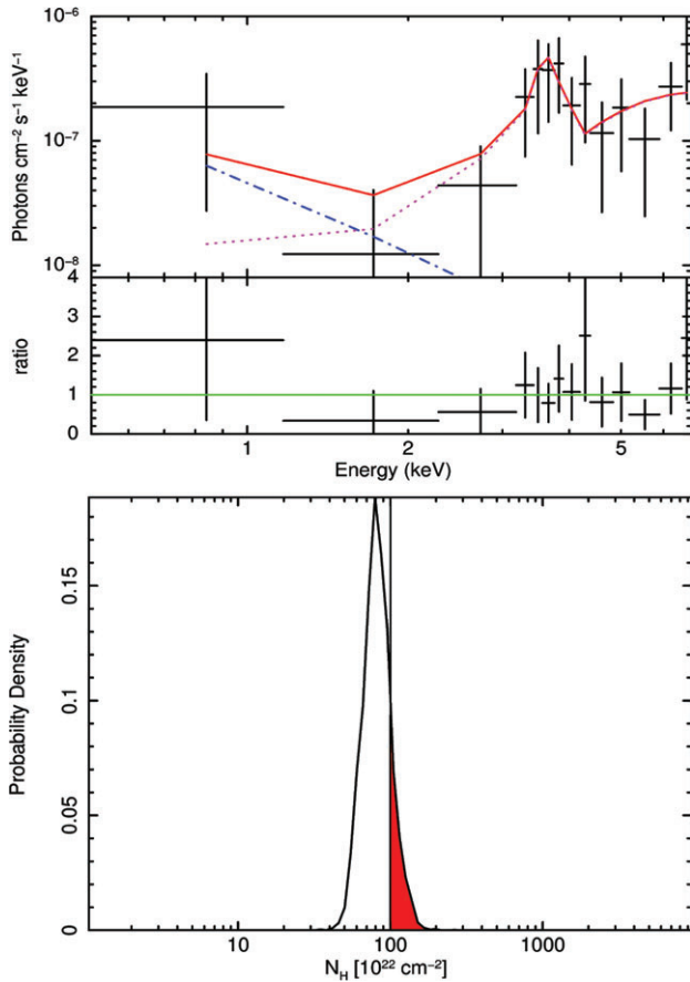
FIGURE 1 (a) Unfolded spectrum and data/model ratio of the CT candidate LID_633 at z = 0.706 . In magenta is shown the BNtorus component, in blue the soft power law, and in red the total. (b) PDF of N_H for the spectrum shown above.
