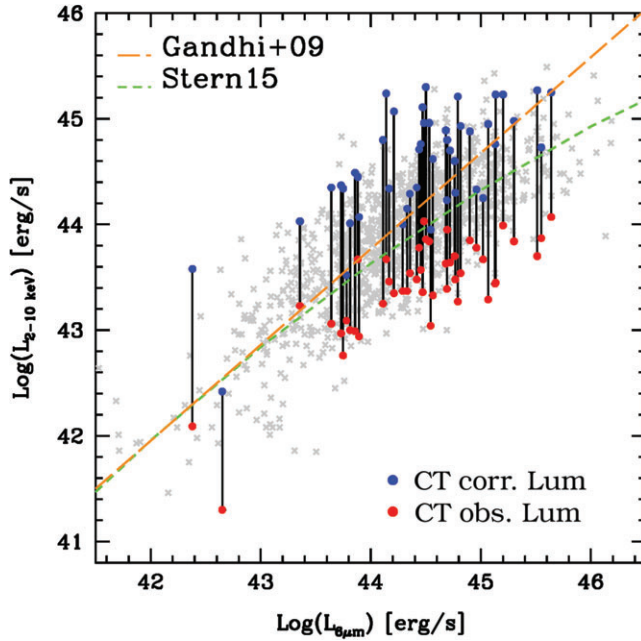
FIGURE 3 Distribution of the AGN mid-IR (6 \mu m) luminosity, as derived from SED fitting, after subtracting the host star-formation emission, and the 2–10 keV luminosity, for the \sim 2,000 sources analyzed in Marchesi et al. (2016a) (gray crosses). Red circles show the observed L_X for the CT candidates, while blue circles show the absorption-corrected L_X . The orange (green) curve shows the relation published in Gandhi et al. (2009) (Stern 2015).
