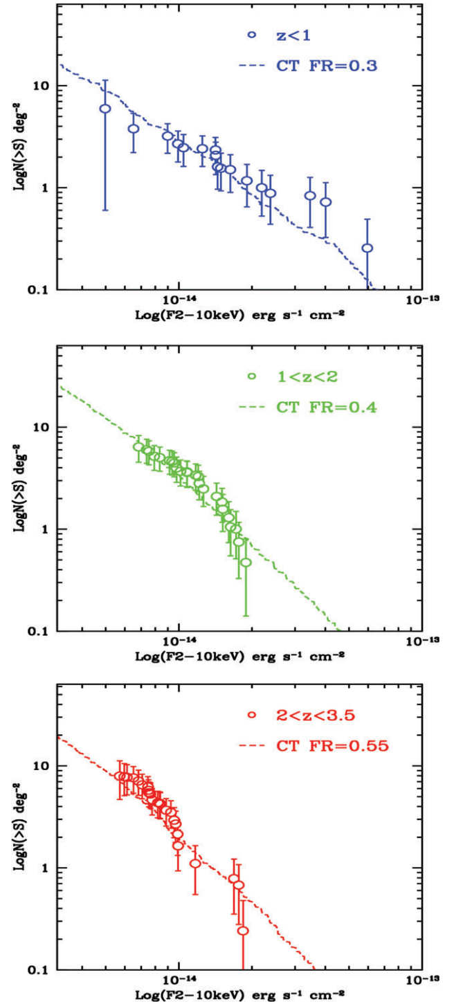
FIGURE 4 Observed log N –log S of CT candidates at z < 1 (top), 1 < z < 2 (center), and 2 < z < 3.5 (bottom), compared with the model of Akylas et al. (2012), with different CT fractions (FR).
