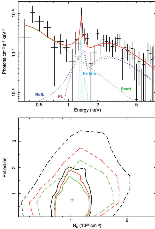
FIGURE 7 (a) Unfolded spectrum of source XID202 from the XMM-CDFS catalog, a CT AGN at z = 3.7 . The different components (primary power law, reflection, Fe line complex, scattered emission) are labeled with different colors. (b) 99, 90, and 68% confidence contours obtained from the XMM-Newton spectrum (thick lines) and from the Chandra one (dotted lines) for N_H and the reflection fraction.
