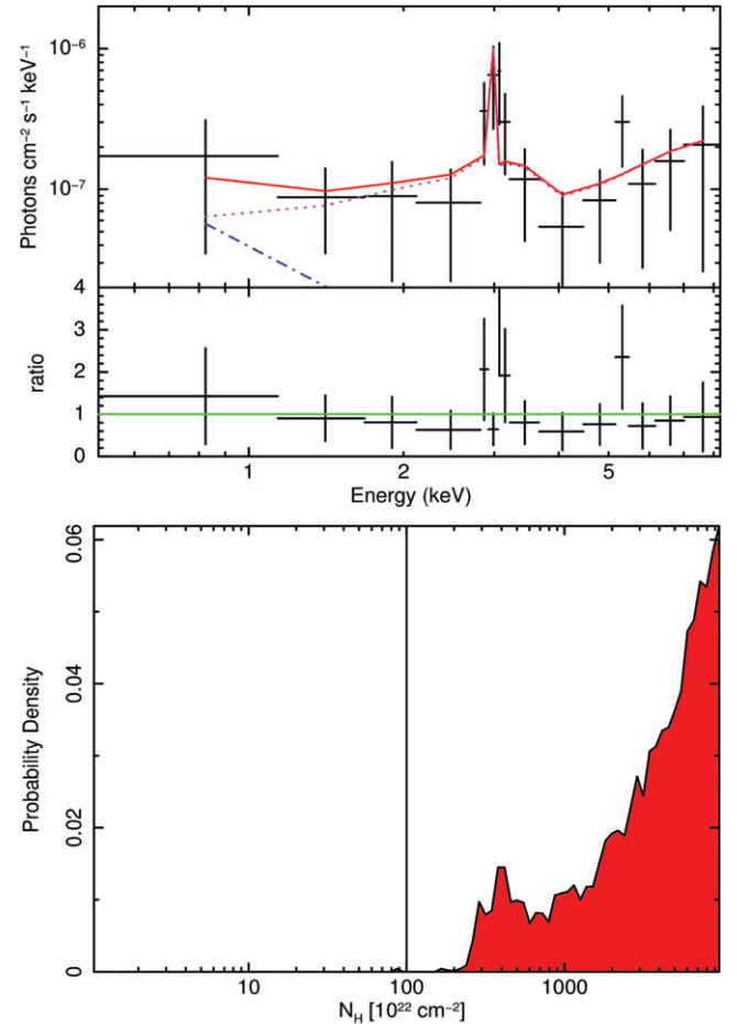
FIGURE 6 Same as Figure 5, for source LID_390.
