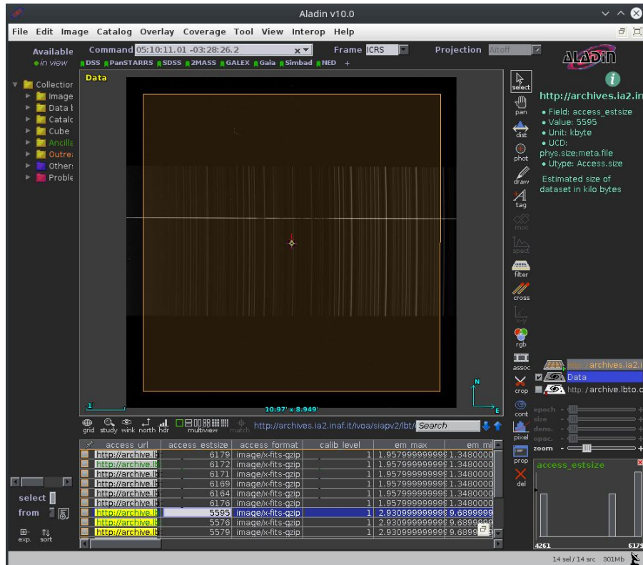
Figure 5: Same as the previous picture but for a spectrum.
