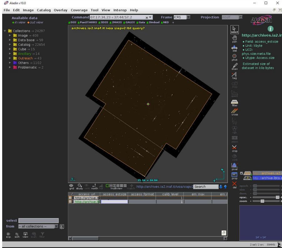
Figure 6: The proposed footprint for raw LBC images displayed in Aladin.
