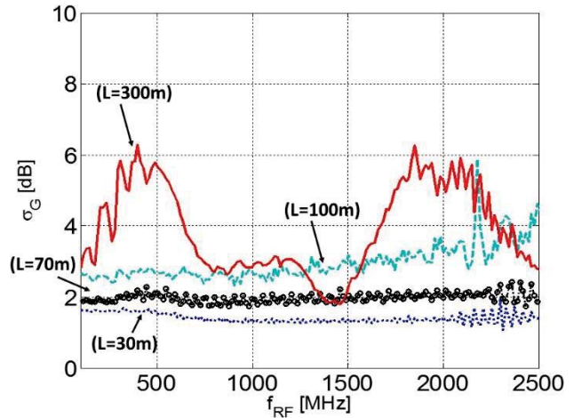
Fig. 4. Typical behaviours of \sigma_G for different SSMF lengths.
