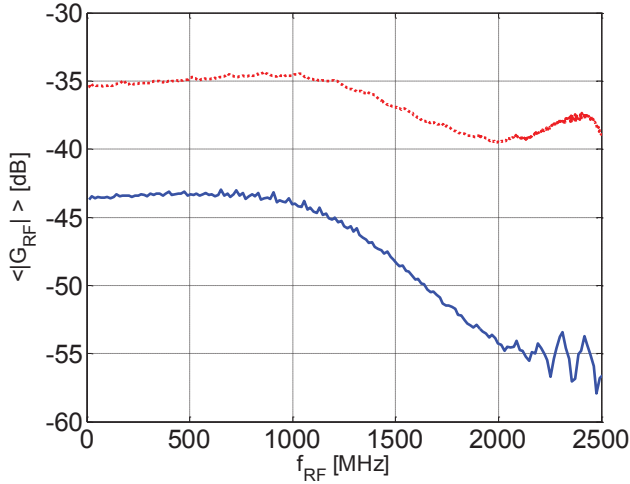
Fig. 5. Comparison of \langle |G_{RF}| \rangle between the MMF-based (red dotted line) and SMF-based (blue solid line) RoF links for 70 m of link length.
