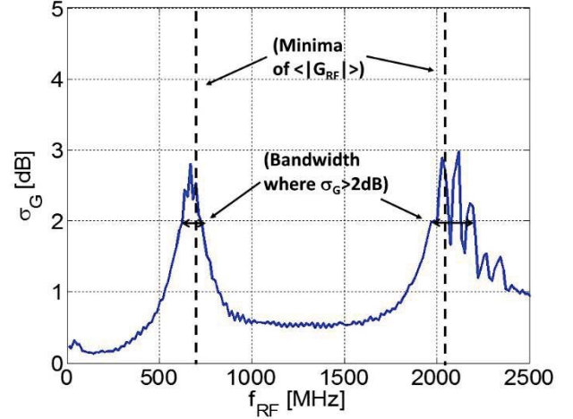
Fig. 3. Experimental measurement of RF gain standard deviation for 300 m of G.652 fiber.
