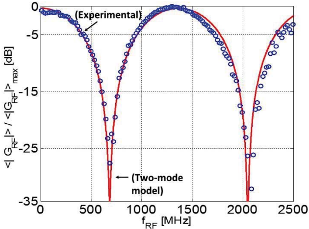
Fig. 1. Effect of intermodal dispersion inside 300m of the SSMF fiber utilized in this work.
