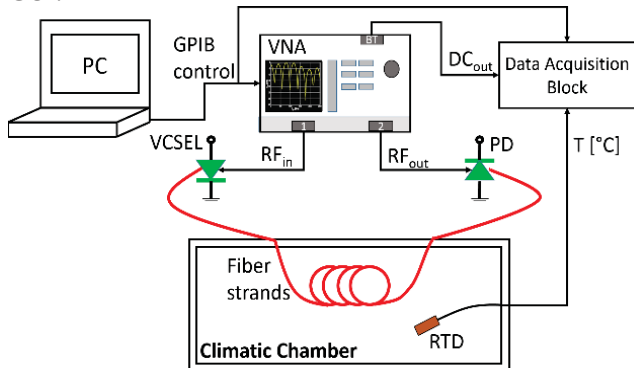
Figure 2: Experimental setup of modal noise effect measurements.
