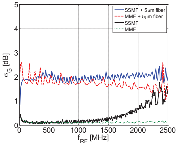
Fig. 6. Comparison in terms of \sigma_G of the MMF-based and SSMF-based 70m RoF links considered, when the fiber is directly connected to the PD and when the SMF5 is placed between them.
