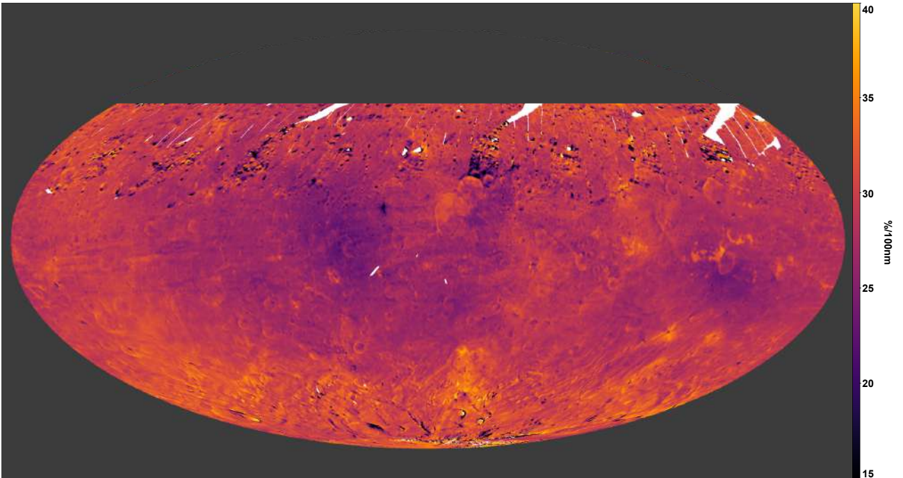
Fig. D.1. Map of the VIR S_{380-465nm} spectral slope without transparency effect and Framing camera context. White areas correspond to missing data.
