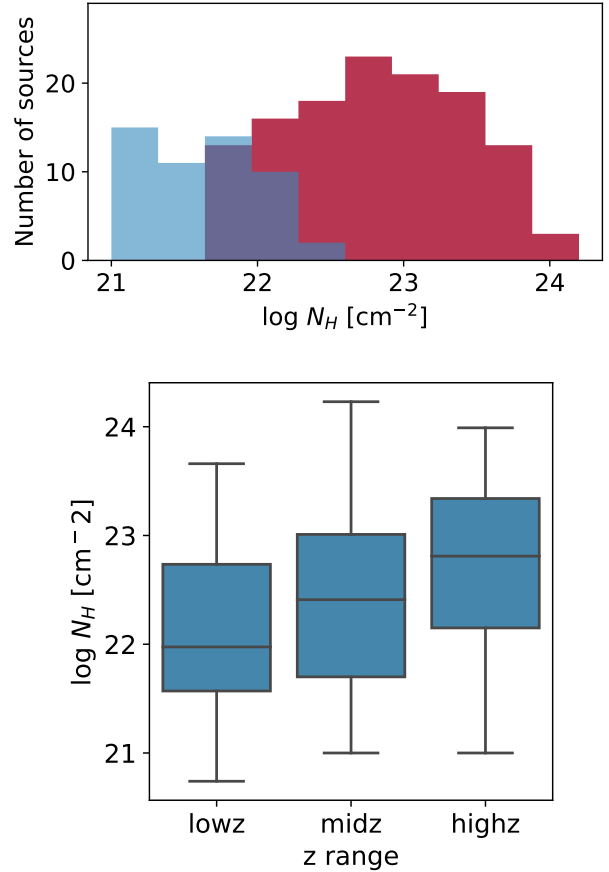
Fig. 3. Upper panel: distribution of best-fit N_H values obtained for all the 180 sources at z > 0.4 . The histogram in red shows the N_H distribution of absorption detected sources, while the blue histogram shows that of the upper limits. We note the limited but uniform sensitivity of our spectra to N_H due to the rest-frame bandpass (see text). Lower panel: box-and-whisker plots of N_H measurements for the lowz, midz and highz groups. Following the normal convention, the box represents the inter quartile range (the middle 50%), the bar in the middle represents the median value, and the whiskers show the range of the minimum and the maximum of the distribution.
