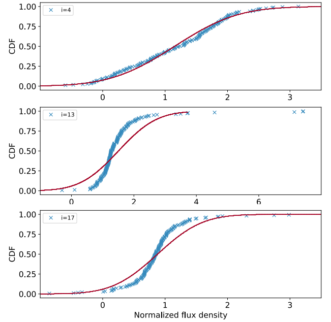
Fig. C.1. CDF of normalised flux density values (blue crosses) of the 180 XMM-CDFS sources in three spectral channels, i = 4 , i = 13 , i = 17 , corresponding to the rest frame energies, 3 keV, 6.3 keV (Fe K band), and 9 keV, respectively. A theoretical curve of the normal distribution which fits the data is overplotted in red in each plot.
