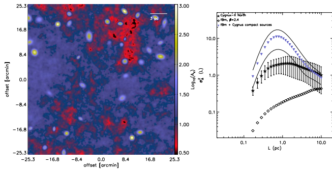
Fig. 20. Left: synthetic column density map generated by reinjecting the compact source extracted from the Cygnus-X North map on top of an fBm image (convolved with a beam with FWHM = 18.2'' ) with \beta = 2.4 . Right: \Delta -variance spectrum of the synthetic models using this approach. The \Delta -variance spectrum of the models is the average over 50 realizations, and the full lines represent the 1\sigma dispersion around the mean. The synthetic \Delta -variance spectra are compared to that of the Cygnus-X North region and to the case of an fBm image with \beta = 2.4 .
