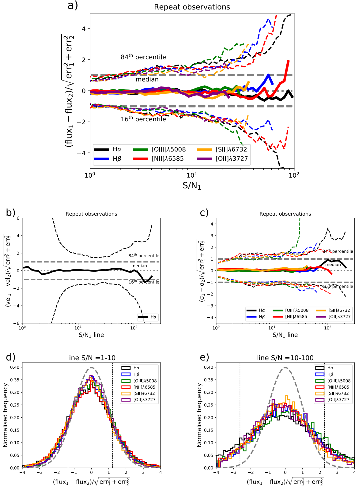
Figure 7. (a) Median flux difference between pairs of repeat observations normalized by rms error, that is, (\text{Flux}_1 - \text{Flux}_2)/(\text{err}_1^2 + \text{err}_2^2)^{1/2} as a function of signal-to-noise ratio ( S/N = \text{Flux}/\text{Error} ) of each line. Different strong emission lines are represented by different colors, as noted in the legend. The 16th and 84th percentiles of the distribution as a function of S/N are shown as dashed lines. If the output errors are correct, the 16th and 84th percentiles of the normalized residual distribution should be \pm 1 . (b) Same as panel (a) but showing the velocity-normalized residuals versus the S/N for the H \alpha line. Only H \alpha is shown because the velocities of all lines are tied. (c) Same as panel (a) but for the velocity dispersion. (d) Distribution of normalized flux residuals in the S/N range [1–10] for six strong emission lines, listed in the legend. The gray dashed line represents the expected distribution assuming Gaussian errors. The black vertical dashed lines are the 16th and 84th percentiles of the H \alpha normalized residual distribution. If the errors are correct, these values should lie at \pm 1 . (e) Same as (b), but for the S/N range [10–100]. Note that in this regime the normalized residual distributions are broader and the errors appear to be underestimated.
