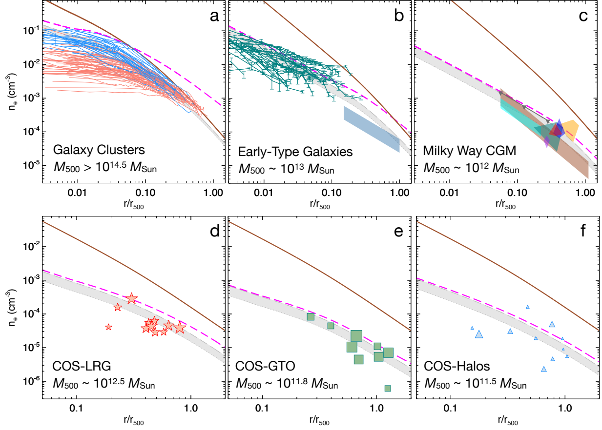
Figure 2: Measurements of electron density in the ambient CGM as a function of radius in units of the cosmological scale radius r_{500} . In each panel, a solid brown line shows the expected electron-density profile without feedback, and a dashed magenta line shows the precipitation limit corresponding to t_{\text{cool}}/t_{\text{ff}} = 10 for a representative potential well in the mass range of that population. Grey regions show hybrid profiles combining the cosmological and precipitation limits for 10 < t_{\text{cool}}/t_{\text{ff}} < 20 [46].
