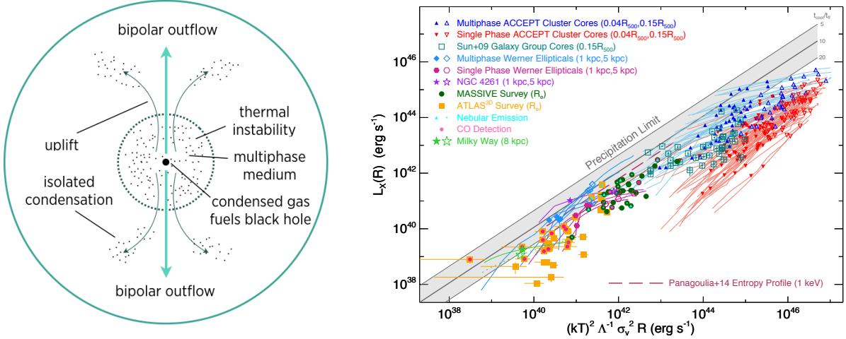
Figure 1: (Left) Schematic representation of precipitation-regulated feedback in a massive galaxy. (Right) Evidence for a pervasive precipitation limit on circumgalactic electron density from observations of X-ray luminosity ( L_X ) within a given radius ( R ) around galaxies more massive than the Milky Way [49].
