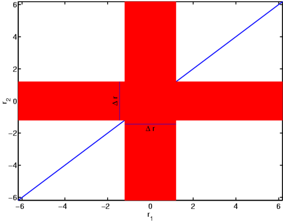
Fig.1 The red area is the region of the r_1, r_2 space excluded by the condition \sigma_1 and \sigma_2 < \sigma_{\text{tgt}} . The width of the two crossing bands, \Delta r , is given by Eq.~(8) and in this case f_{\text{DAE,excl}} \sim 0.35 .
