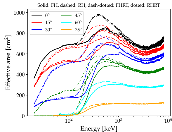
Figure 6 Simulations of the off-axis effective area as a function of the energy, for different solutions in terms of mask thickness and side shielding thickness. Note above \sim 150 keV that the surrounding structures become transparent and the detector becomes mostly isotropic (response dominated by the cosine effect). FH = Full Height collimator with 0.2 W thickness, RH = Reduced Height collimator (half of FH), RT = Reduced Thickness of the collimator and of the coded mask.
