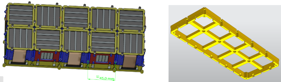
Figure 15 Left: Super-Module arrangement (view from the radiation entrance side); right Super-Module frame (bottom view, the Modules are mounted on the upper part of the frame, and screwed together via the vertical holes than can be seen in the central rib and in the periphery of the frame, the horizontal holes will be used to connect the frame together)
