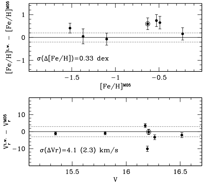
Figure 6. Comparison between the [\text{Fe}/\text{H}] and V_r estimates obtained in this work (t.w.) and M05b, for the seven stars in common. The encircled dot correspond to a star with molecular bands in its UVES spectrum, whose metallicity is classified as tentative by M05b. In the lower panel, the standard deviation value reported in parentheses refers to the sub-sample from which the outlier at \Delta V_r \simeq 10 \text{ km s}^{-1} has been removed. The dotted lines enclose the range 0.0 \pm 0.2 dex in the upper panel, and 0.0 \pm 3.0 \text{ km s}^{-1} in the lower panel.
