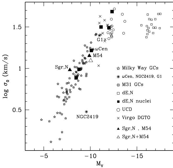
Figure 21. Sgr,N and M54 (filled triangles) in the M_V vs. \sigma plane (see Evstigneeva et al. 2007). Both systems lie on the locus common to globular clusters, dE nuclei, Dwarf-Globular Transition Objects (DGTO Hasegan et al. 2005), and, possibly, UCDs. The same is true for their combination (Sgr,N+M54, open triangle), i.e., for a system having luminosity equal to the sum of the luminosities of M54 and Sgr,N and having \sigma as estimated from an integrated spectrum obtained with a 1'' slit from the distance of the Virgo cluster of galaxies ( \sigma \simeq 12.4 \text{ km s}^{-1} ). Data for galactic globulars are from Mackey & van den Bergh (2005, M_V ) and Pryor & Meylan (1993, \sigma ); for M31 globulars we took integrated magnitudes from the Revised Bologna Catalog (Galletti et al. 2004) and \sigma from Djorgovski et al. (1997); data for dE and dE,N are from Geha et al. (2002, 2003); UCDs data are from Drinkwater et al. (2003) and Evstigneeva et al. (2007); data for DGTO are from Hasegan et al. (2005). Some remarkable bright clusters have been labeled, for reference (see Federici et al. 2007).
