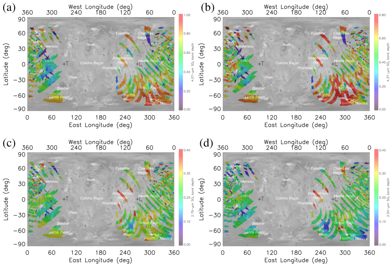
Figure 4. Spatial distribution of the depth of the strongest absorption bands diagnostic of SO 2 frost, revealed between 2.5 and 4.5 \mu\text{m} . (a) Map of band depth for the main SO 2 band, centered at 4.07 \mu\text{m} . (b) Map of band depth for the 4.37- \mu\text{m} signature. (c) Map of band depth for the 2.79- \mu\text{m} absorption. (d) Map of band depth for the 2.54- \mu\text{m} feature. The maps derived from the weighted averages of JIRAM-derived band depths are transparently superimposed onto an optical mosaic of the Io surface, to facilitate association with some of the major geologic formations. Color bars have different ranges in different panels because the absorption bands at 4.07 and 4.37 \mu\text{m} are much stronger than the bands at 2.79 and 2.54 \mu\text{m} . In all maps presented in this figure and in the following ones, the horizontal axes express both east and west longitudes, so as to enable a quick comparison with past results, which used west longitudes, but also facilitate a comparison with the data that will be acquired by future space missions such as JUICE and Europa Clipper, which may favor eastward longitudes. The “+T” and “+L” symbols mark the apex of the trailing and leading hemispheres, respectively.
