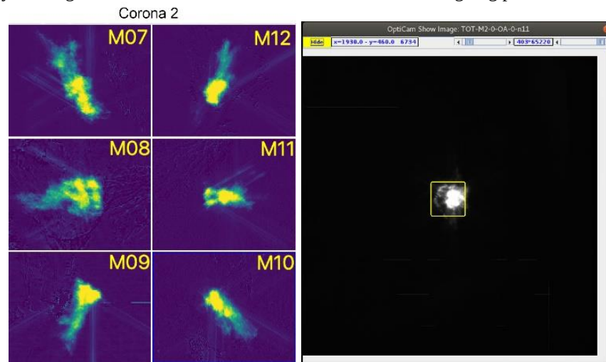
Figure 7. Left: images produced by the M1 mirrors of corona two. Right: the result of the alignment procedure. The linear dimensions of yellow square are 7×7 mm corresponding to the linear dimensions of a pixel of the ASTRI Mini-Array camera (courtesy of ASTRI project).
