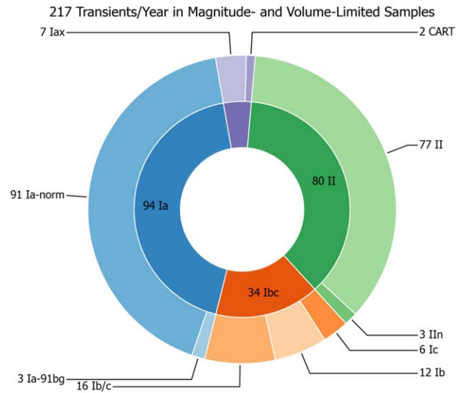
Figure 5. Same as Figure 4, but for YSE SNe per year meeting the criteria of our volume- or magnitude-limited surveys, <250 Mpc or r < 18.5 mag (a magnitude at which we expect to be able to obtain spectroscopic classifications). We predict 94 SNe Ia, 34 SNe Ib/c, 77 SNe II, and 3 SNe IIIn per year. SN models are from PLAsTiCC (Kessler et al. 2019 and references therein). We note that PLAsTiCC templates for certain models, including a subset of SN II and Ib/c, were not given subtypes. Sixty-one transients (36% of the volume-limited sample) are both more distant than 200 Mpc and fainter than \sim 18.5 , the limits of the ZTF “Census of the Local Universe” (CLU) and magnitude-limited samples.
