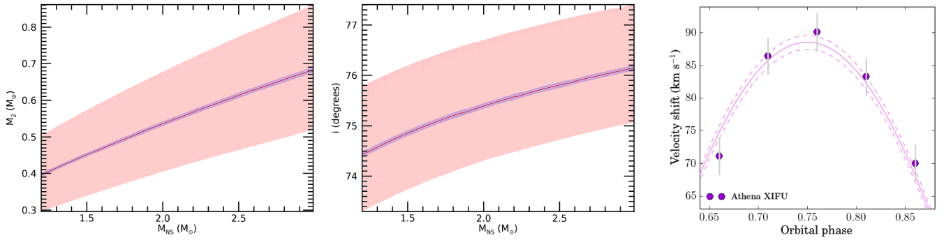
Figure 5. Left and centre panels: Constraints on the orbital inclination ( i ), NS ( M_{\text{NS}} ) and companion star masses ( M_2 ) derived from the mass function (equation 1) and the eclipse duration (equation 3), under the assumption that the companion star fills its Roche lobe (equation 4). The pink and violet areas show the region allowed by the current and future ( Athena ) uncertainties. Right panel: Determination of the semi-amplitude of the radial velocity curve through a 100 ks Athena XIFU observation. A zoom on a small part of the radial velocity curve is shown, in order to exhibit the small uncertainties. K_1 will be precisely constrained to ( K_1 = 89.0 \pm 0.9 \text{ km s}^{-1} ).
