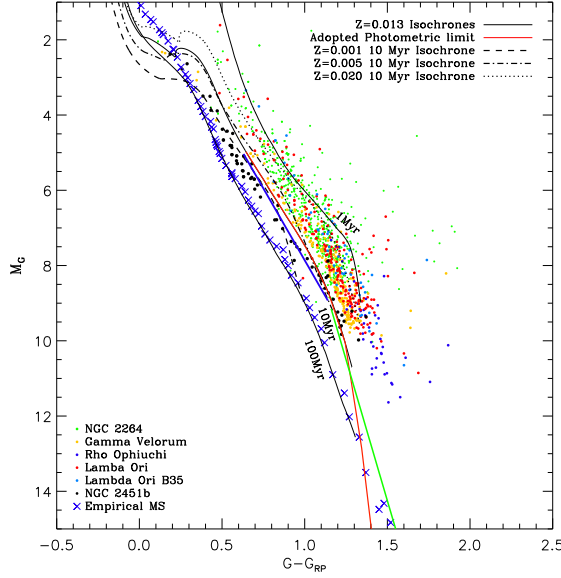
Fig. 1. CAMD of YSOs of some representative young clusters with membership probabilities >0.90 assigned by combining spectroscopic and Gaia EDR3 criteria (Jackson et al. 2022). Blue x symbols trace the empirical sequence by Pecaute & Mamajek (2013). Members of the clusters Gamma Velorum (18 Myr old) and NGC2451b (50 Myr old) are also shown. Black solid lines are the theoretical solar metallicity PISA isochrones while the red solid line is the complete photometric limit adopted in this work including the low mass extrapolation. Dashed, dashed-dotted and dotted lines are the 10 Myr isochrones at different metallicities. Blue and green solid lines represent the limits described by the equations 2 and 3.
