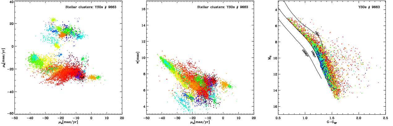
Fig. 7. Proper motions in RA and Dec, parallaxes, and CAMDs of the groups of YSOs associated with the Sco OB2 association. The symbol colours are as in Fig. 6. Three representative solar metallicity isochrones from the Pisa models are also shown as solid lines in the right panels .
