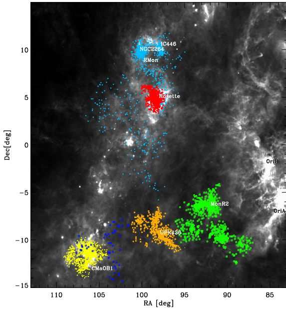
Fig. 8. Spatial distribution in equatorial coordinates of the YSOs associated with NGC 2264, NGC 2244, Mon R2, CMA OB1, and UPK 436. YSOs are overplotted on an IRIS 100 \mu m image (Miville-Deschênes & Lagache 2005). For clarity, Orion members have not been plotted.
