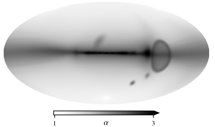
Fig. 8. Template for the noise estimation parameter, \alpha_\phi . The noise model is introduced in Eq. (5), the template is based on the Galactic electron model derived by Yao et al. (2017).
