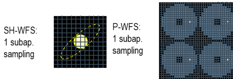
Figure 2. Difference in pixels occupation for a SH-WFS ( left ) and a P-WFS ( right ), in the LGS sensing case. In the SH-WFS focal plane, re-imaged spots have different angular sizes: the smallest (solid line) and the largest (dashed line) spots are reported.
