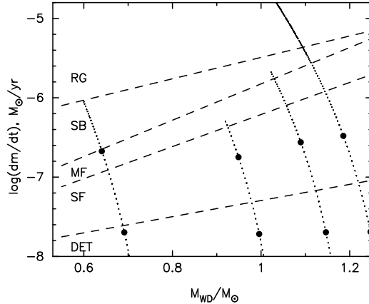
Figure 1. Helium burning regimes in the layer of accreted He depending on the mass of the accretor M_{WD} and the accretion rate \dot{M}_{acc} [5]. Dashed lines mark the boundaries of the zones in which detonation (DET), strong (SF) and weak (MF) flashes, steady burning (SB) occur. In the RG-region of the diagram, extended envelopes around WDs are formed. Dotted lines show the evolutionary tracks of the stars considered in this paper. Filled circles on the tracks correspond to the age of the system 10^5 and 10^6 years.
