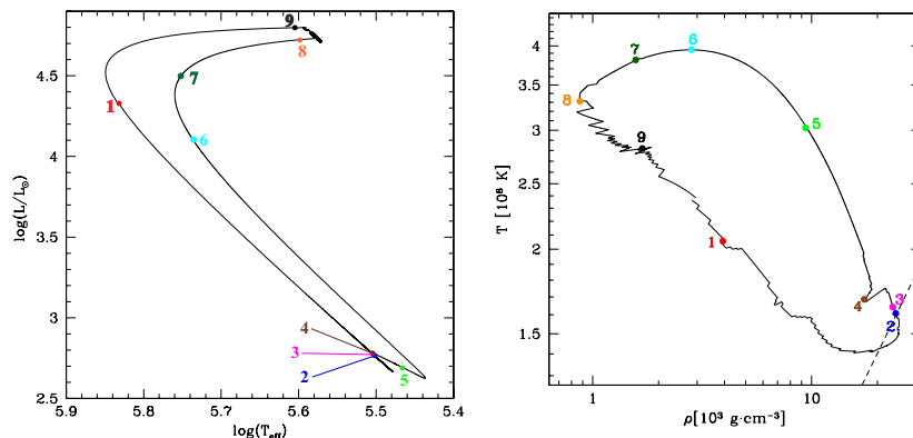
Figure 2. Left panel – evolutionary track of accreting WD in (1.02 \pm 0.3) M_\odot system in the HRD. Right panel – evolution of temperature and density in the He-burning zone. 1 – resumption of accretion after previous flash, t_{9-1}=28 yr; 2 – He-ignition, t_{1-2}=870 yr; (2-3) – rapid increase of nuclear energy release, t_{2-3}=5.93 yr; (3-4) – thermonuclear runaway, formation of convective zone, t_{3-4}=214 day; 5 – maximum outward extension of convective zone, T \approx 3 \cdot 10^8 K, activation of ^{22}\text{Ne}(\alpha, n)^{25}\text{Mg} reaction, onset of neutron-isotopes nucleosynthesis, t_{4-5}=314 day; 6 – temperature maximum in the He-burning zone ( 3.8 \cdot 10^8 K), t_{5-6}=7.5 day; (6-8) – active burning of ^{22}\text{Ne} , t_{6-8}=3.57 yr; (8-9) – RLOF stage, t_{8-9}=8.63 yr.
