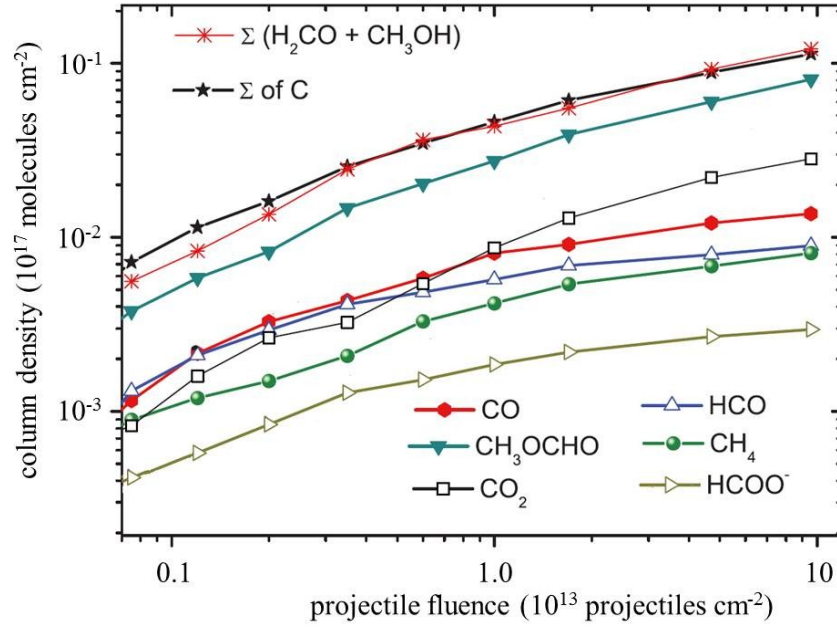
Figure 9. The total and partial carbon column densities of a \text{H}_2\text{O}:\text{H}_2\text{CO}:\text{CH}_3\text{OH} (100:2:0.8) ice mixture irradiated by 220 MeV ^{16}\text{O}^{7+} ions as a function of projectile fluence. The partial values were determined according to the carbon stoichiometry (data taken from de Barros et al 2014a).
