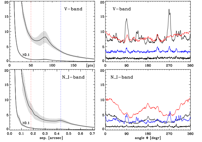
Fig. 9. Azimuthally averaged radial profiles ct_{\text{n6}}(\rho) (left) and azimuthal profiles ct_{\text{n6}}(r, \phi) for r = 50, 80, 120 and 180 pix (right) corresponding to \rho = 0.18'', 0.29'', 0.43'', and 0.65'' , respectively for the PSFs of HD 183143 shown in Fig. 8. Also indicated as gray shading are the standard deviations of the azimuthal points \sigma(ct_{\text{n6}}(r, \phi)) . The location of the azimuthal cuts are indicated in the ct_{\text{n6}}(r) -panels and in Fig. 8.
