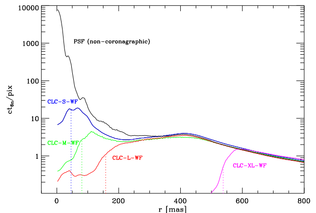
Fig. 17. Normalized radial profiles ct_{66}(r) for the I_PRIM coronagraphic images in Fig. 16 of \alpha Hyi taken with the small S (blue), medium M (green), large L (red), and extra-large XL (magenta) focal plane stops. Also plotted is the non-coronagraphic PSF profile. The dotted lines indicate the nominal mask radii.
