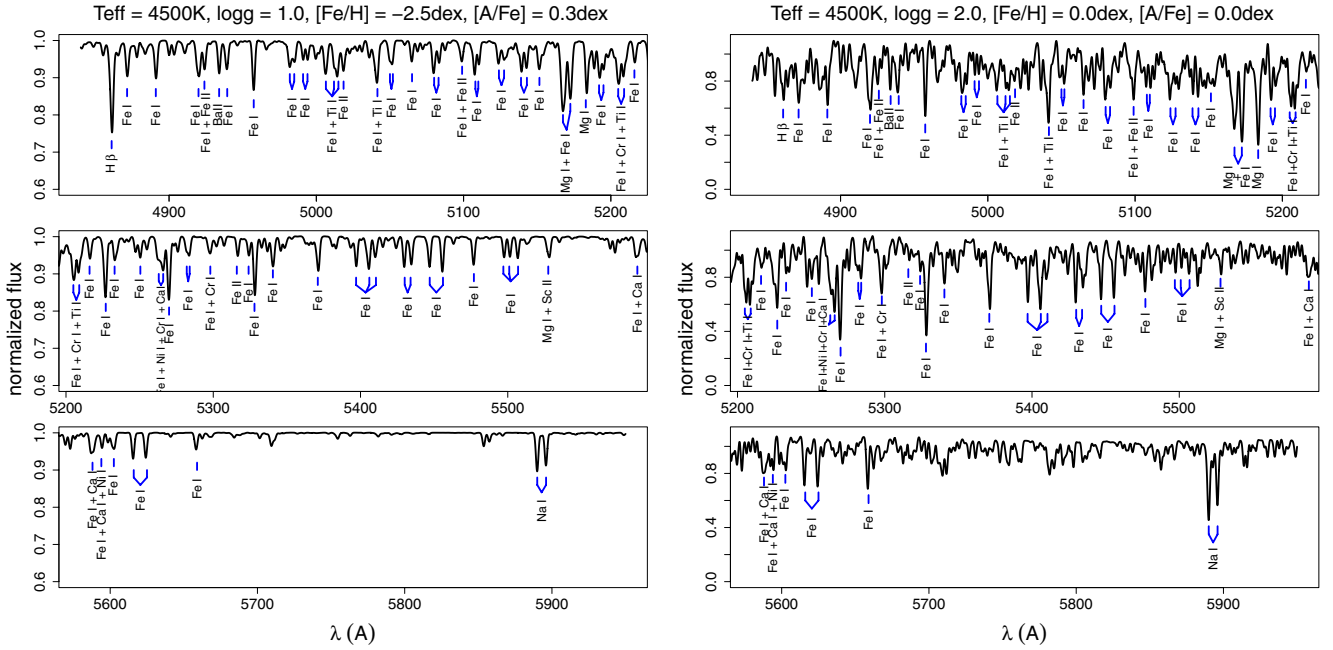
Fig. 3. Most important atomic lines in each strong spectral feature with FORS2 resolution ( R \sim 2000 ). The most important molecular band in this region is MgH around \lambda = 5165 Å, on top of the MgI triplet lines. The left panel shows a metal-poor red giant star from the library of Coelho et al. (2005) , the right panel shows a metal-rich. The left panels were zoomed in the y -axis direction for better visualization.
