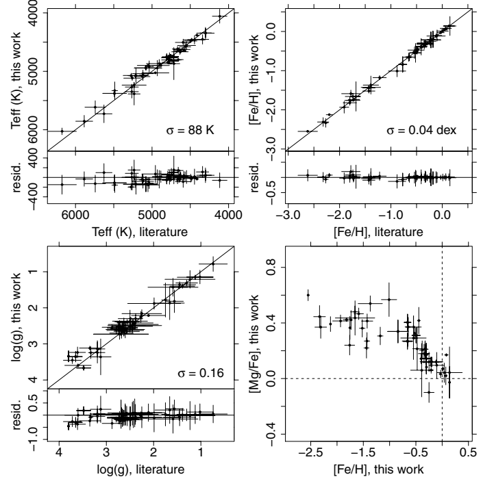
Fig. 8. Comparison of the parameters determined with PASTEL catalogue average values for the well-known stars presented in Table 4. These plots endorse the ETOILE code for atmospheric parameter determination for red giant stars in the optical spectral region. Only stars with \sigma_{T_{\text{eff}}} < 200 K, \sigma_{\log(g)} < 0.5 , \sigma_{[\text{Fe}/\text{H}]} < 0.2 from the PASTEL catalogue were selected as good-quality candidates to validate the method. Below the plots of T_{\text{eff}} , \log(g) , and [\text{Fe}/\text{H}] we plot the residuals, the residual dispersion is displayed in the respective plots.
