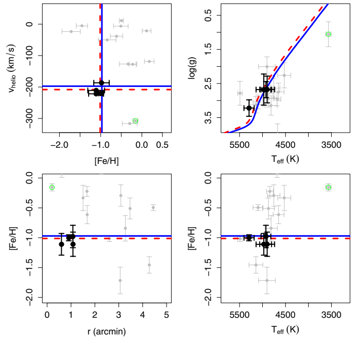
Fig. 17. Same as Fig. 13 for NGC 6558.
