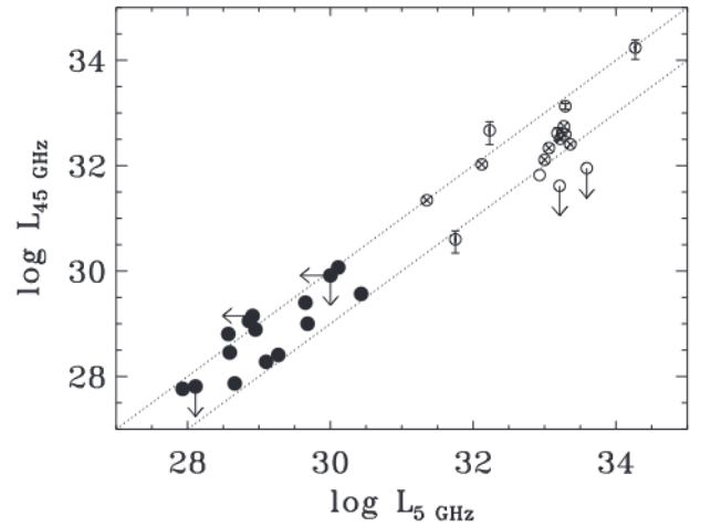
Figure 6. The 5-GHz radio core luminosities versus the 45-GHz luminosity ( \text{erg s}^{-1} \text{ Hz}^{-1} ). The filled points are the 15 RQQs, the empty points are the RLQs with available VLA Q-band data and the crossed empty circles are the RLQs with the 45-GHz flux densities extrapolated from their radio spectra. The RLQs are typically \sim 1000 more luminous than the RQQs at both 5 GHz and 45 GHz. The dotted lines are drawn to visualize a scatter of a factor of 10. The scatter of RQQs ( \sigma = 0.29 ) is smaller than that of RLQs ( \sigma = 0.41 ).
