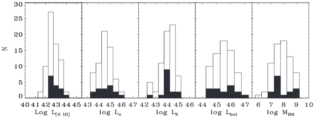
Figure 1. Distribution of the [O III] line, optical (4400 Å), X-ray (2–10 keV), bolometric luminosities (in erg s ^{-1} ) and BH masses (in M_{\odot} ) of the whole PG RQQ sample (71 objects). The filled histograms represent the distribution of the 15 PG RQs studied in this work. The KS tests confirm that the 15 sources are representative of the entire PG RQQ sample.
