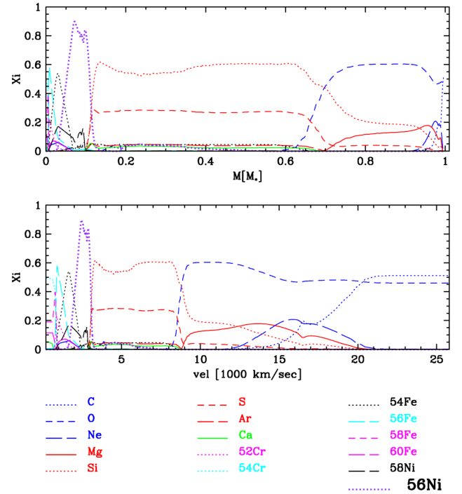
Fig. 25. Same as Fig. 24 but showing the overall abundance structure at large times as a function of mass coordinate (top) and expansion velocity (bottom). It is very similar to the subluminal model for SN 1999by and consistent with the chemical structure based on our abundance tomography given in Table 3. In addition, we show the initial ^{56}\text{Ni} \rightarrow ^{56}\text{Co} \rightarrow ^{56}\text{Fe} at the time of the explosion (purple dotted line).
