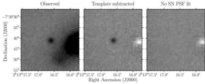
Fig. 2. g -band imaging of SN 2016hbk and its host galaxy, before (left) and after (middle) subtracting the host galaxy template using hotpants integration in SNOOPY. This example shows how the subtracted image is clean enough to perform PSF fitting, as shown in the right panel where the SN PSF has been removed. A small residual of the galaxy core is shown on the middle and right panels (white blob), however it does not affect SN PSF fitting.
