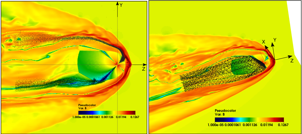
Figure 3. 3D maps of selected particles superimposed on the 3D structure of the magnetic field in the BSPWN. On the left we show a 2D cut in the y - z plane, at x = 0 of the BSPWN color-coded according to the strength of the magnetic field in code units. Blue-cyan regions locate the position of the polar and equatorial currents. Over-imposed is the projection on the same plane of the position of particles injected in the polar regions \theta = [0, 10]^\circ and \theta = [170, 180]^\circ , corresponding to the two PSR spin-axes pointing respectively toward and away from the PSR kick velocity (along positive z ). On the right we show a 3D axonometric-projection of the BSPWN sliced along the y - z half-plane and x - z , again color-coded according to the strength of the magnetic field in code units, together with the 3D positions of particles injected in the equatorial region \theta = [85, 95]^\circ .
