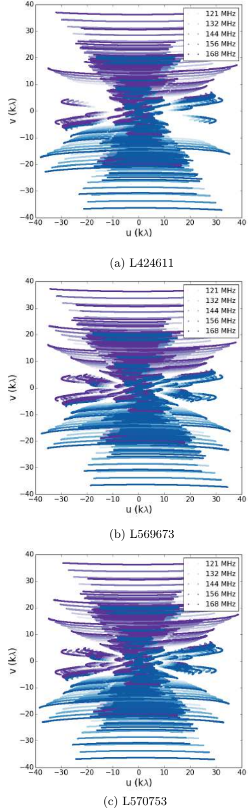
Fig. 1. uv coverage of the data in k\lambda for the three observations. Panel a is for observation of L424611, panel b for L569673, and panel c for L570753. The shades of purple represent five different frequency bands corresponding to those at 121 MHz (lightest), 132 MHz, 144 MHz, 156 MHz, and 168 MHz (darkest). The conjugate points are plotted in blue.
