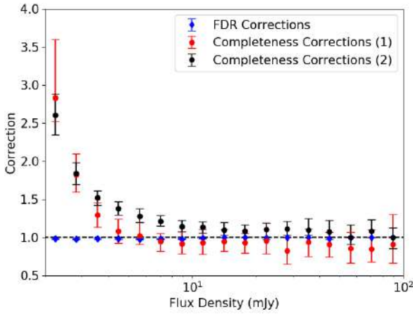
Fig. 12. Correction factors calculated and then applied to the source counts from the catalogue using the methods described in Sects. 6.1 and 6.2: FDR corrections (blue) and completeness/resolution correction using Method 1 (red) and Method 2 (black).
