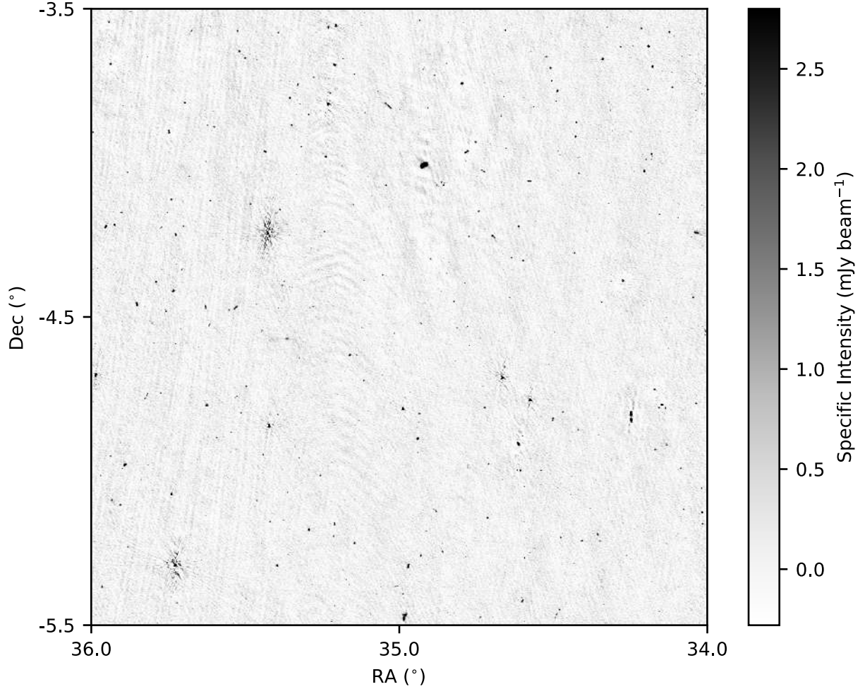
Fig. 4. Image of the central 4 deg 2 of the field, containing ~600 sources. This has the same flux scale as Fig. 3, ranging between -\sigma_{\text{cen}} and 10\sigma_{\text{cen}} , where \sigma_{\text{cen}} is the central rms of the image, which is 0.28 mJy beam -1 . This zoomed-in image allows the presence of multi-component sources in this field to be seen.
