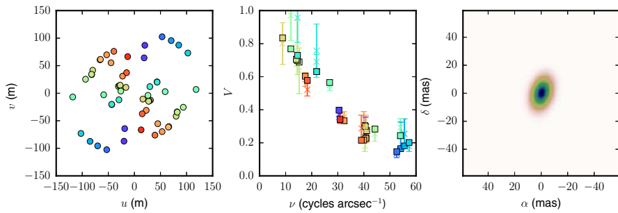
Fig. 11 The mid-IR geometry of the high-mass YSO V921 Sco. Left panel The uv-plane coverage of the VLT/IRAM observations with the MIDI instrument. Middle panel The visibility amplitude as a function of spatial frequency. The color of the points corresponds with the position angle of the measurement. Right panel Geometrical representation of the visibility function which consists of a compact 2D Gaussian combined with 1D Gaussian halo. Adapted from Boley et al. (2013) (reproduced with permission from Astronomy & Astrophysics, © ESO)
