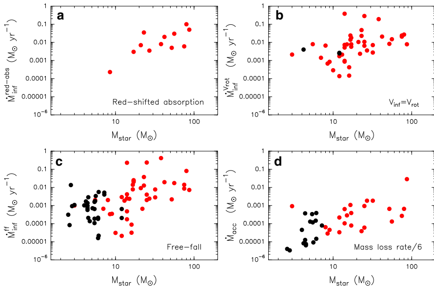
Fig. 15 Mass infall and accretion rate as a function of M_{\star} , where the infall rate has been estimated a from red-shifted absorbed line profiles, \dot{M}_{\text{inf}}^{\text{red-abs}} (see Eq. 3), for the rotating structures around HM (proto)stars for which red-shifted absorption has been detected; b assuming that the infall velocity is equal to the rotation velocity, \dot{M}_{\text{inf}}^{\text{Vrot}} (see Eq. 4), for the rotating structures around HM (red dots) (proto)stars (Table 2) and for the few IM (black dots) (proto)stars (Table 1) with rotation velocity information available; and c assuming that all the material in the rotating structure will collapse in a free-fall time t_{\text{ff}} , \dot{M}_{\text{inf}}^{\text{ff}} (see Eq. 5), for all the IM (black dots) and HM (red dots) (proto)stars (Tables 1, 2). The mass accretion rate \dot{M}_{\text{acc}} ( d ) has been estimated from the outflow mass loss rate \dot{M}_{\text{out}} (see Eq. 6), for those IM (black dots) and HM (red dots) (proto)stars for which interferometric observations of molecular outflows are available (Tables 1, 2)
