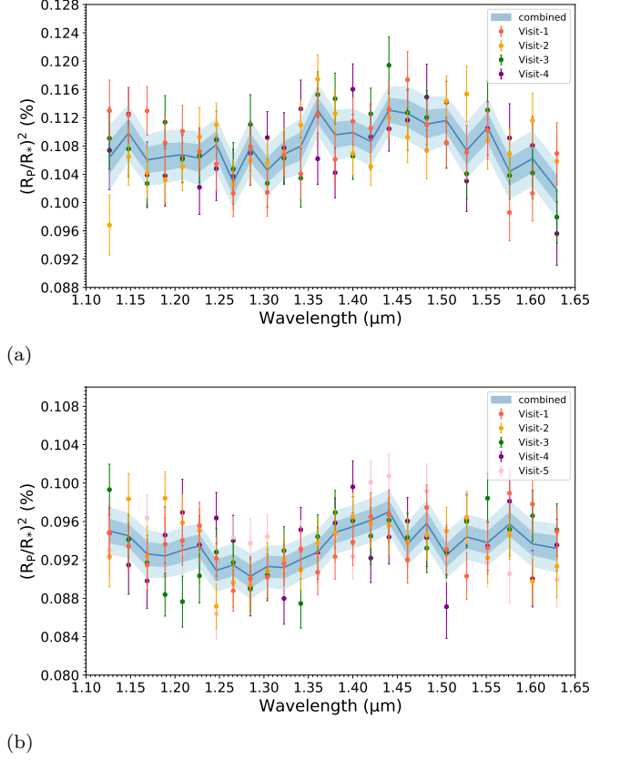
Figure 4. Spectra per visit and final weighted average with 1\sigma and 2\sigma uncertainty ranges for HD 106315 c (a) and HD 3167 c (b).
