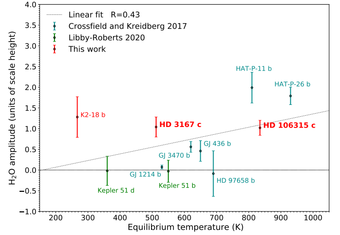
Figure 10. Normalized H 2 O amplitude in units of scale height with respect to equilibrium temperatures. Blue points are from Crossfield & Kreidberg (2017) and green points are from Libby-Roberts (2020) . Red points are computed using the method described in Crossfield & Kreidberg (2017) and spectra obtained in this work and from Tsiaras et al. (2019) for K2-18 b. The dotted line corresponds to a linear fit. The correlation coefficient was found to be lower than in Crossfield & Kreidberg (2017) , 0.43 compared to 0.83.
