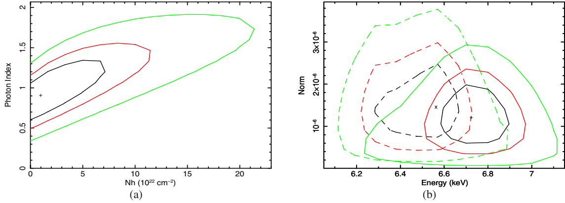
Fig. 1. a) Confidence contour plot for the photon index against the column density using an absorbed PL model. b) Confidence contour plot showing the normalization against energy of the Fe K \alpha emission line for the PN (solid lines) and MOS (dashed lines) spectrum. The contours are at 68%, 90%, and 99% confidence levels for two interesting parameters.
