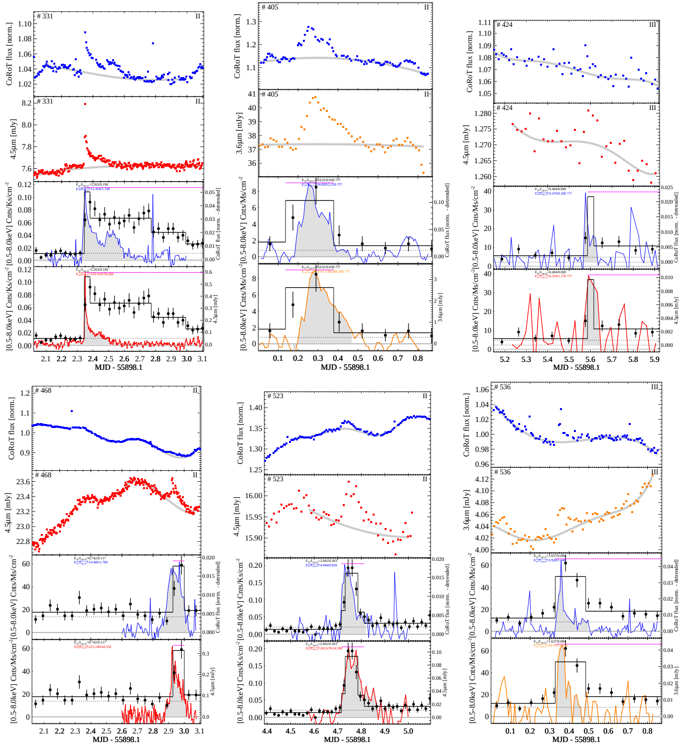
Fig. B.1. Lightcurves of all X-ray flares with counterparts in the optical and/or mIR bands. See caption of Fig. 2 for a full description of the content of each panel.
