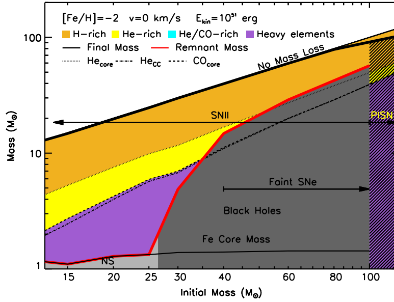
Fig. 24g Same as Figure 24a but for models with initial metallicity [\text{Fe}/\text{H}] = -2 .
