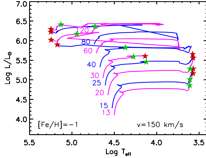
Fig. 10e Same as Figure 10d but for models with initial rotation velocity v = 150 \text{ km/s} .
