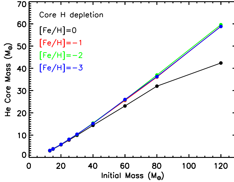
Fig. 5 He core mass at core at core H depletion as a function of the initial mass for non rotating models with initial metallicities [\text{Fe}/\text{H}] = 0 (black line), [\text{Fe}/\text{H}] = -1 (red line), [\text{Fe}/\text{H}] = -2 (green line) and [\text{Fe}/\text{H}] = -3 (blue line).
