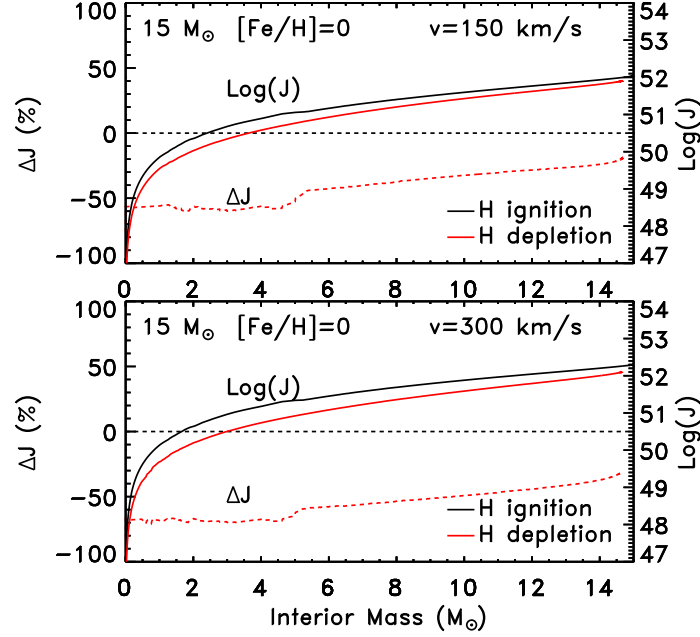
Fig. 9a Angular momentum as a function of the enclosed mass for a 15 M_{\odot} model with initial metallicity [\text{Fe}/\text{H}]=0 and with initial rotation velocities v = 150 \text{ km/s} (upper panel) and v = 300 \text{ km/s} (lower panel). The black and red solid lines refer to the stage corresponding to the core H ignition and core H depletion, respectively (their scale is on the right y-axis). In each plot it is also reported the percentage variation of the angular momentum between the core H ignition and core H depletion (red dotted lines - left y-axis).
