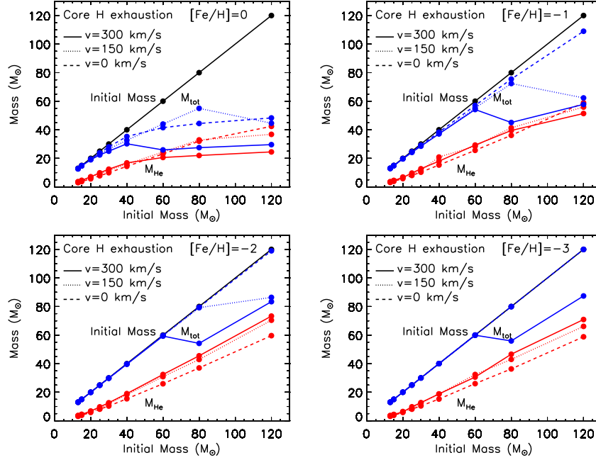
Fig. 8 Total mass (blue lines) and He core mass (red lines) at core H exhaustion as a function of the initial mass, for models with metallicity [\text{Fe}/\text{H}] = 0 (upper left panel), [\text{Fe}/\text{H}] = -1 (upper right panel), [\text{Fe}/\text{H}] = -2 (lower left panel) and [\text{Fe}/\text{H}] = -3 (lower right panel). The dashed, dotted and solid lines refer to models with initial rotation velocity v = 0, 150, 300 km/s, respectively.
