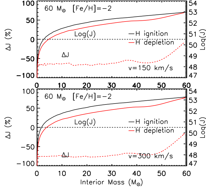
Fig. 9d Same as Figure 9b but for an initial metallicity [\text{Fe}/\text{H}] = -2 .
