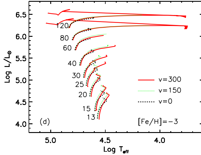
Fig. 6d Same as Figure 6a but for metallicity [\text{Fe}/\text{H}]=-3 .
