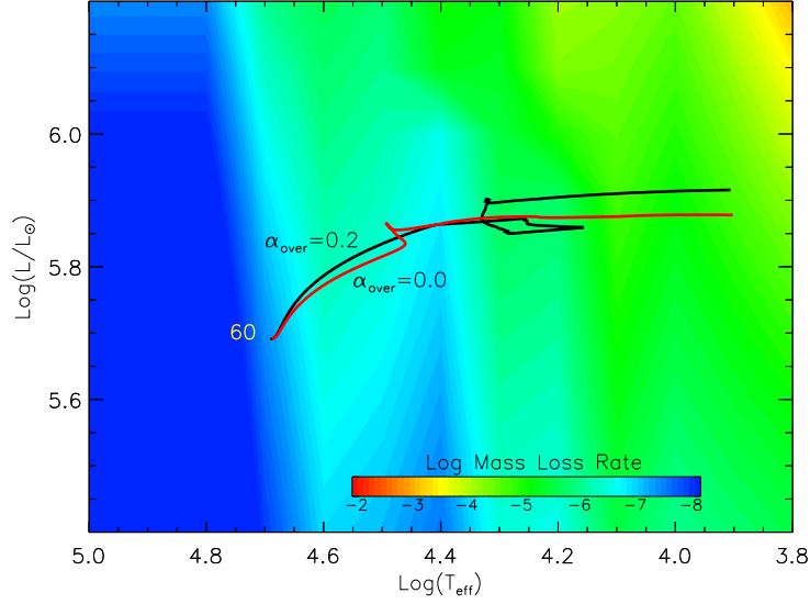
Fig. 3 Evolutionary tracks in the HR diagram of two non rotating 60 M_{\odot} models of solar composition during core H burning. The black line refers to the model computed assuming 0.2 H_p of core overshooting while the red line refers to the model computed without any convective core overshooting. The mass loss rate corresponding to the various regions of the HR diagram follows the color codes reported in the color bar.
