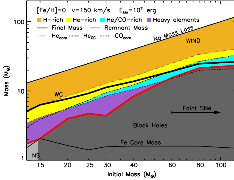
Fig. 24b Same as Figure 24a but for models with initial rotation velocity v = 150 km/s.
