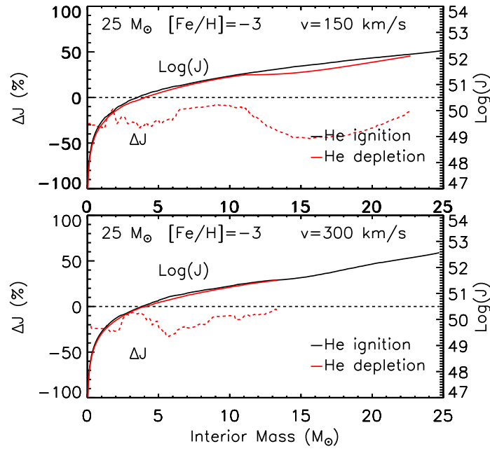
Fig. 14e Same as Figure 14d but for a 25 M ⊙ model.
