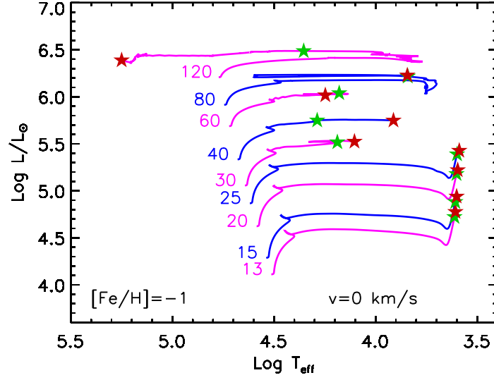
Fig. 10d Same as Figure 10a but for models with initial metallicity [\text{Fe}/\text{H}] = -1 .
