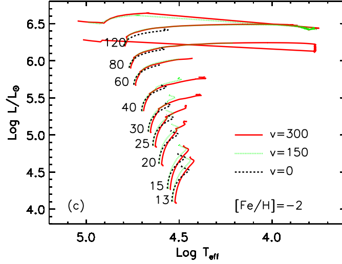
Fig. 6c Same as Figure 6a but for metallicity [\text{Fe}/\text{H}]=-2 .
