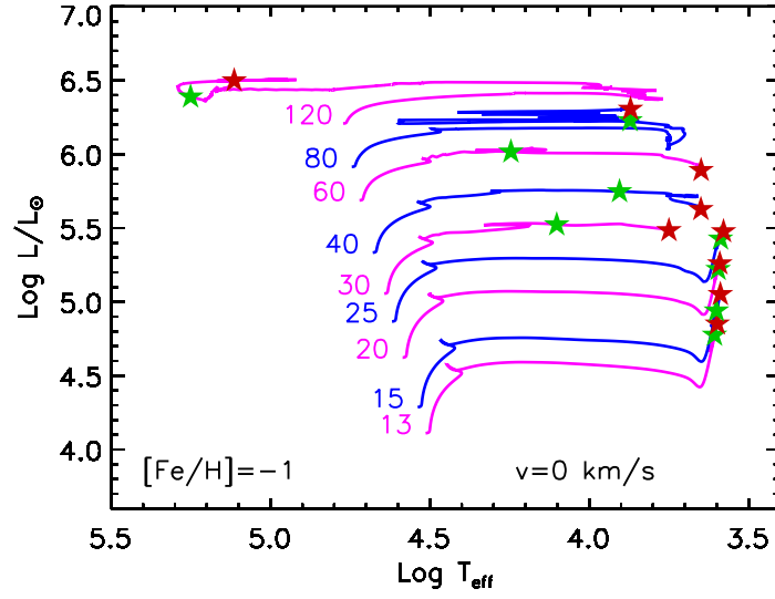
Fig. 22d Same as Figure 22a but for models with initial metallicity [\text{Fe}/\text{H}] = -1 .
