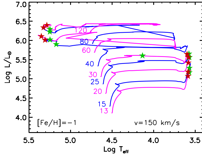
Fig. 22e Same as Figure 22d but for models with initial rotation velocity v = 150 \text{ km/s} .
