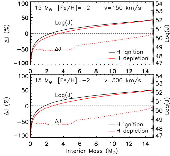
Fig. 9c Same as Figure 9a but for an initial metallicity [\text{Fe}/\text{H}] = -2 .
