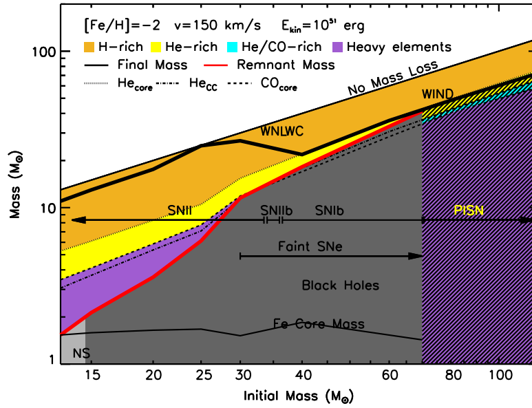
Fig. 24h Same as Figure 24g but for models with initial rotation velocity v = 150 \text{ km/s} .
