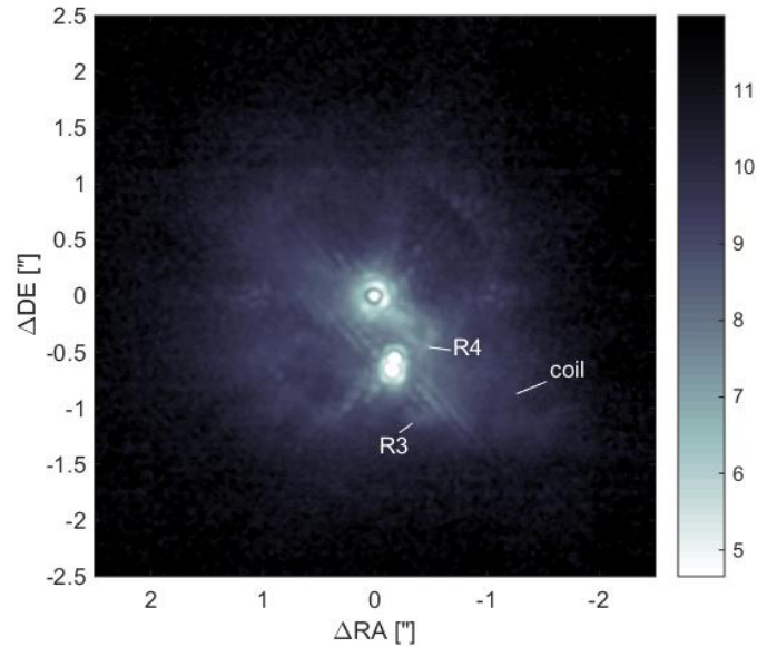
Fig. 5. Coronagraphic K 1-band image of T Tauri displayed in a logarithmic color scale showing the flux level in magnitude per arcsecond 2 . T Tauri N is masked by the ALC coronagraph.
