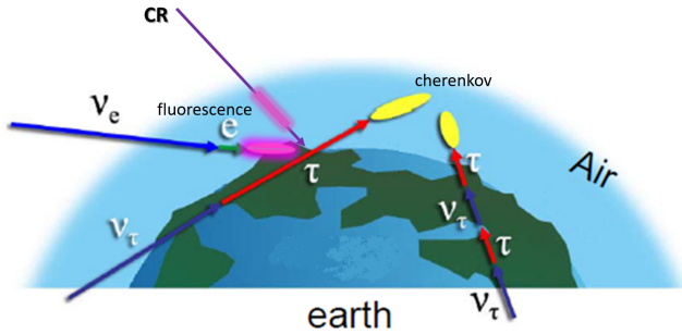
Figure 1: Artistic representation of some particles that can produce fluorescence and Cherenkov light when they interact with the Earth's atmosphere.
