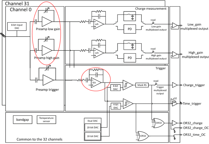
Figure 4: General block scheme of the CITIROC with the changes to be made for RADIOROC highlighted by red ovals.
