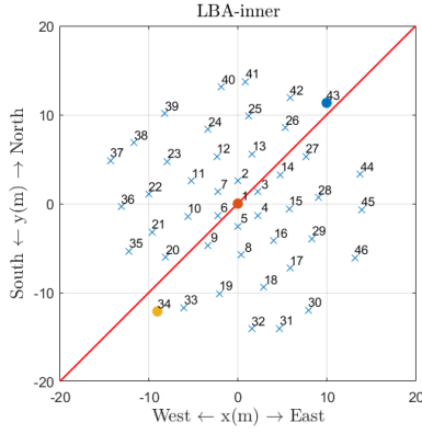
Fig. 4. LBA-inner array: antennas distribution (crosses), antenna index (number from 1 to 46; antennas 47 and 48 are used for calibration purposes and are located outside this area) and nominal UAV trajectory (red line) are shown. Colored circles indicate the antennas whose amplitudes are shown in Fig. 5.
