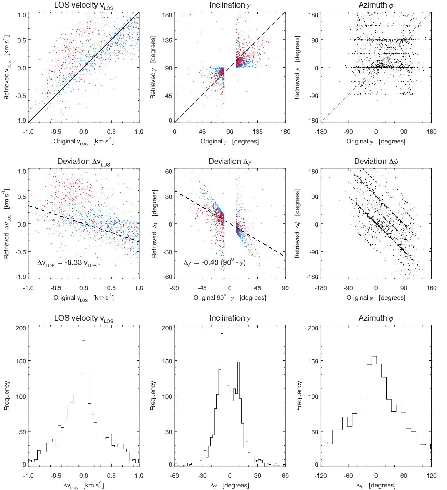
Figure A3. Same as in Figure A2, but for v_{\text{LOS}} , \gamma , and \phi . Blue (red) points refer to original atmospheric models with B < 100 G ( B > 100 G). The dashed lines overplotted on the deviation of v_{\text{LOS}} and \gamma represent a linear fit to the data.
