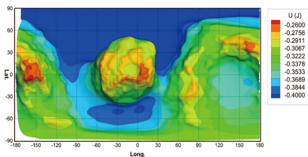
Figure 4. A Mercator projection of the gravitational potential ( U ) of comet 67P.
