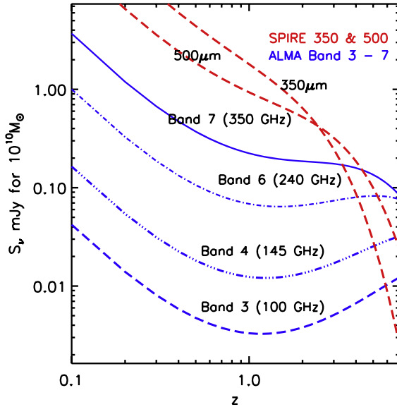
Figure 18. The expected continuum fluxes for the ALMA bands at 100, 145, 240, and 350 GHz and for SPIRE 350 and 500 \mu\text{m} for M_{\text{ISM}} = 10^{10} M_\odot derived using the empirical calibration \alpha = 6.7 \times 10^{19} (Scoville et al. 2016) and an emissivity power-law index \beta = 1.8 and including the RJ departure coefficient \Gamma_{\text{RJ}}(25 \text{ K}) . Since the point-source flux sensitivities of ALMA in the four bands are quite similar, the optimum strategy is to use Band 7 out to z \sim 2 –3 above z = 3 . Lower frequency ALMA bands are required to avoid large uncertainties in the RJ correction.
