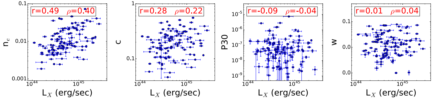
Figure 16. Correlations between the X-ray luminosity and some of the morphological parameters computed within R_{500} . The correlation coefficient decreases from the left to the right.
