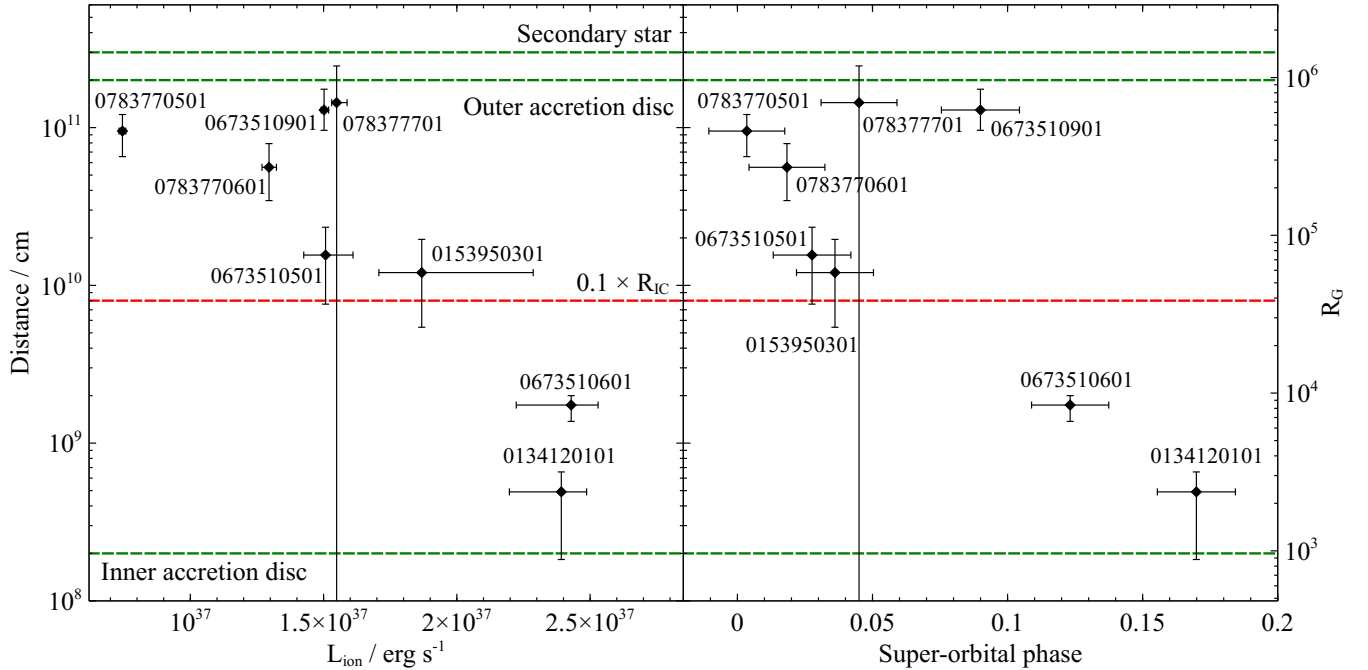
Figure 12. The estimate of the maximum distance of photoionised absorption from the ionising source versus the ionising luminosity (left subplot) and the super-orbital phase (right subplot). The green horizontal lines show the positions of the inner and outer edges of the accretion disc, and the distance of the secondary star from the primary. The red dashed line shows the approximate position of the minimum wind launching radius if the wind is powered by Compton heating of the accretion disc.
