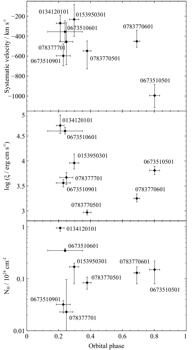
Figure 10. Top plot: Systematic velocity of the ionised absorber with respect to the orbital phase during each observation. Middle plot: Ionisation parameter of the absorber versus the orbital phase during each observation. Bottom plot: Column density of the absorber versus the orbital phase during each observation.
