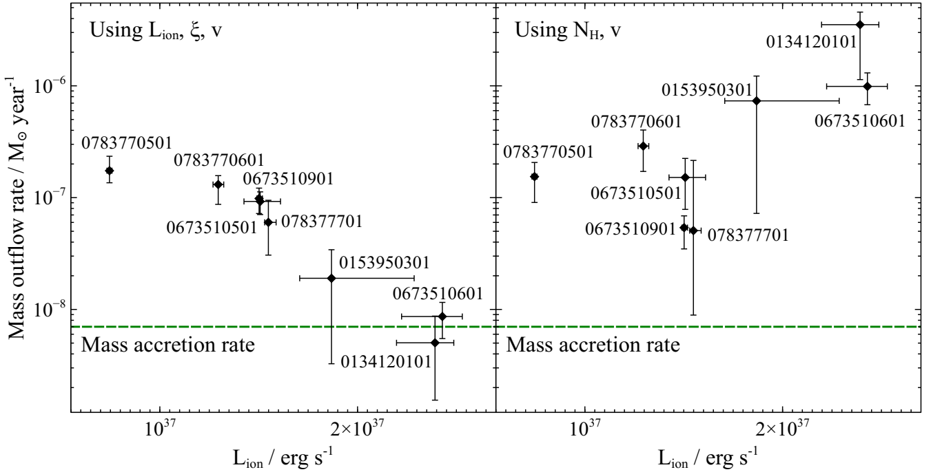
Figure 13. The mass outflow rate of the wind for each observation. The estimate in the left plot was made using the ionising luminosity of the source, the ionisation parameter and the velocity of the material. The estimate in the right plot was made using the column density and the velocity of the wind. The green horizontal lines show the mass accretion rate through the accretion disc (Boroson et al. 2007).
