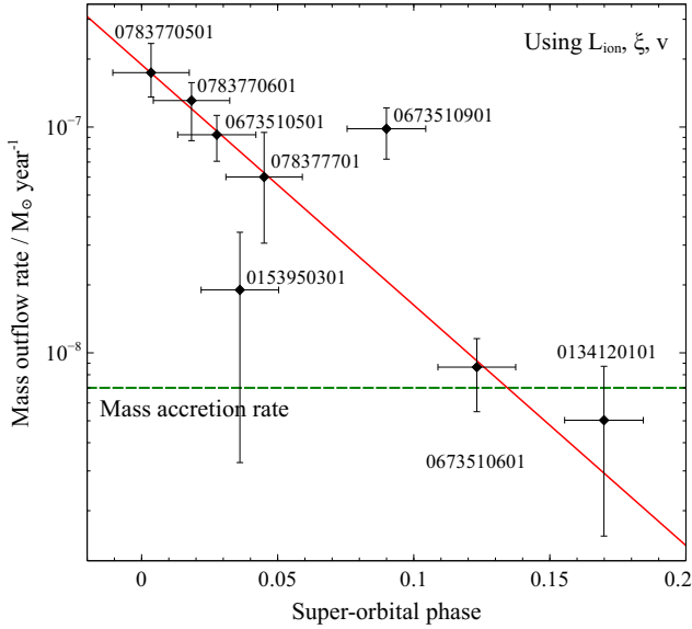
Figure 14. Wind mass outflow rate versus the super-orbital phase of each observation. The red line shows the best log-linear fit to the data, excluding observations 0153950301 and 0673510901 and treating them as outliers.
