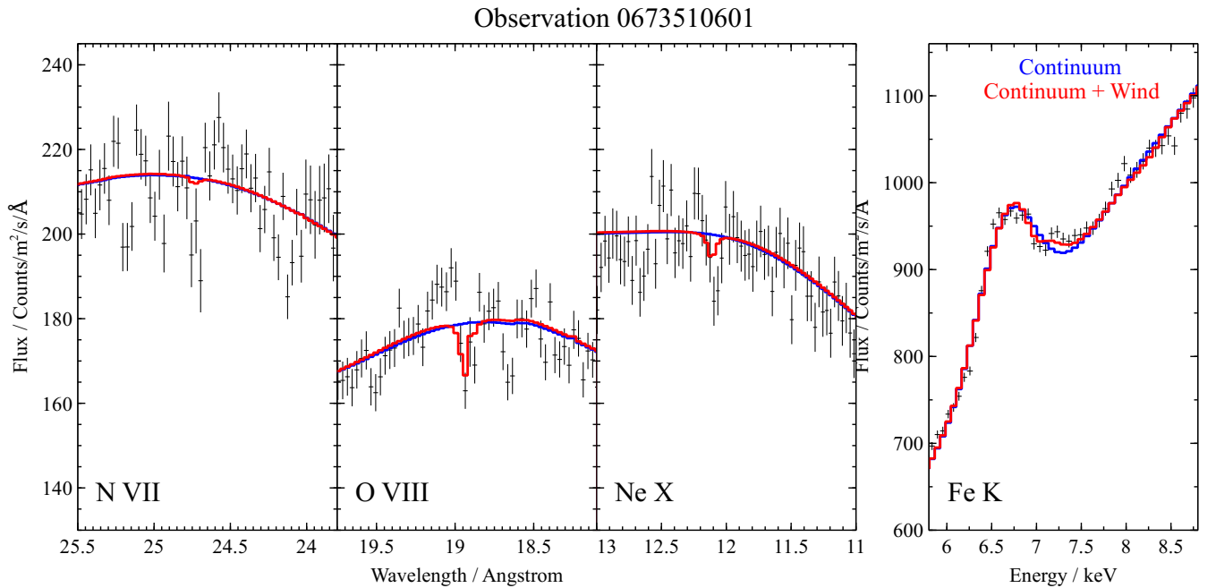
Figure 4. Same plot as Fig. 3 but for observation 0673510601.
