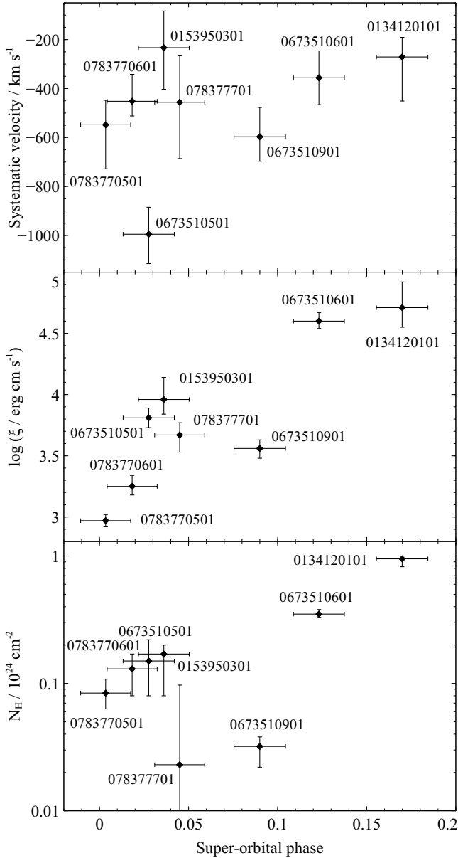
Figure 11. Top plot: Systematic velocity of the ionised absorber with respect to the super-orbital phase during each observation. Middle plot: Ionisation parameter of the absorber versus the super-orbital phase during each observation. Bottom plot: Column density of the absorber versus the super-orbital phase during each observation.
