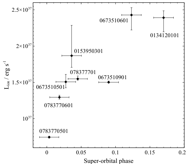
Figure 8. Extrapolated 1–1000 Ryd ionising luminosity for each of the high state observations versus the super-orbital phase.
