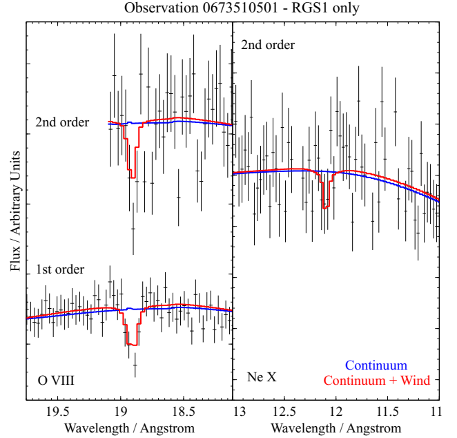
Figure A2. The best-fitting spectral models for observation 0673510501 using only RGS 1 first and second order data. Only the O VIII and Ne X bands are shown as the NVII signature is insignificant in this case. The best-fitting baseline continuum is shown in blue and the final wind solution in red.
