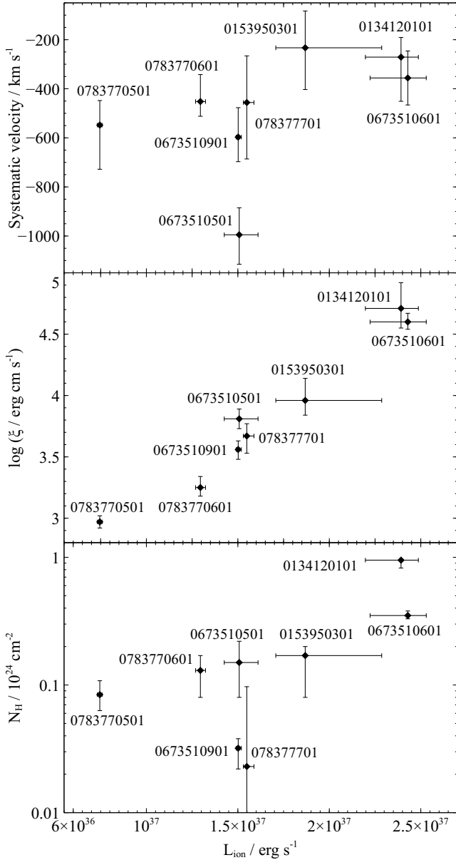
Figure 9. Top plot: Systematic velocity of the ionised absorber with respect to the extrapolated 1-1000 Ryd ionising luminosity of Her X-1 for each observation in the high state. Middle plot: Ionisation parameter of the absorber versus the extrapolated 1-1000 Ryd luminosity for each observation in the high state. Bottom plot: Column density of the absorber versus the 1-1000 Ryd luminosity for each observation.
