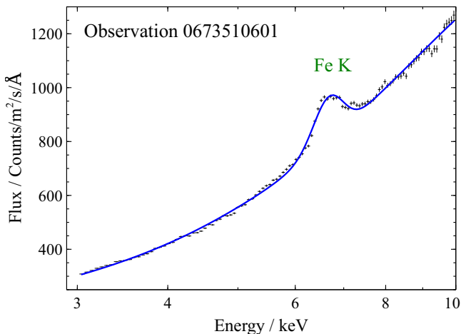
Figure 1. Example 3-10 keV spectrum of Her X-1 with XMM-Newton pn instrument (Obs ID 0673510601). The broadband shape is reasonably well fitted with a Comptonisation model plus a broad iron line at \sim 6.6 keV.
