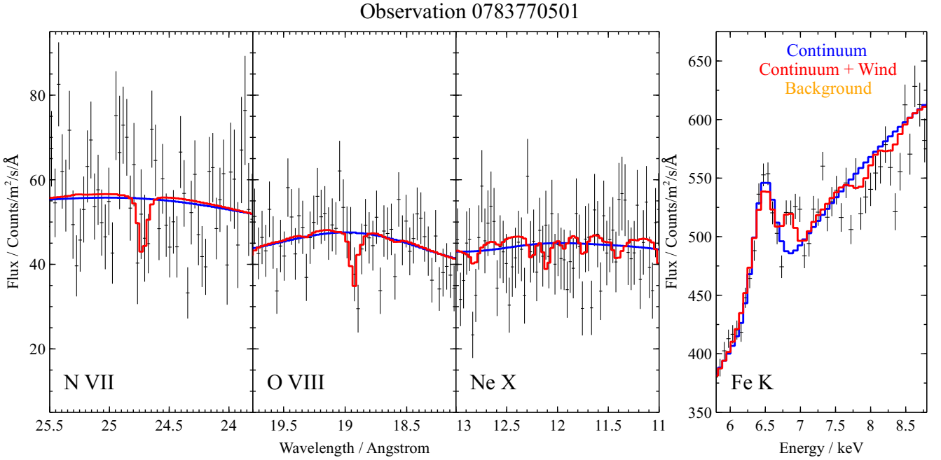
Figure 6. Same plot as Fig. 3 but for observation 0783770501.
