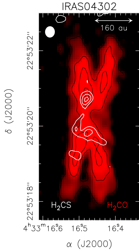
Fig. 6. Spatial distribution (moment 0) maps (white contours) of the o-H 2 CS(7 1,6 –6 1,5 ) line (see Fig. 1), overlaid on the o-H 2 CO(3 1,2 – 2 1,1 ) reported by Podio et al. (2020a) , in black contours and red scale. Symbols are as in Figure 1.
