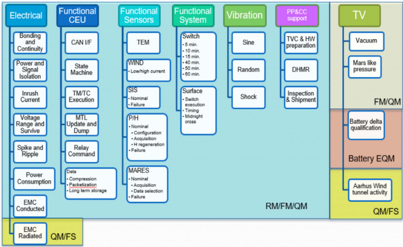
Fig. 6. Test activity conducted on the different DREAMS models.
