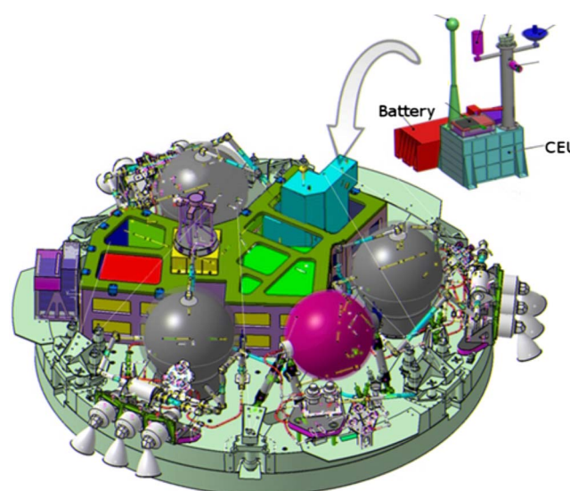
Fig. 1. DREAMS experiment position on board Exomars EDM landing platform.
