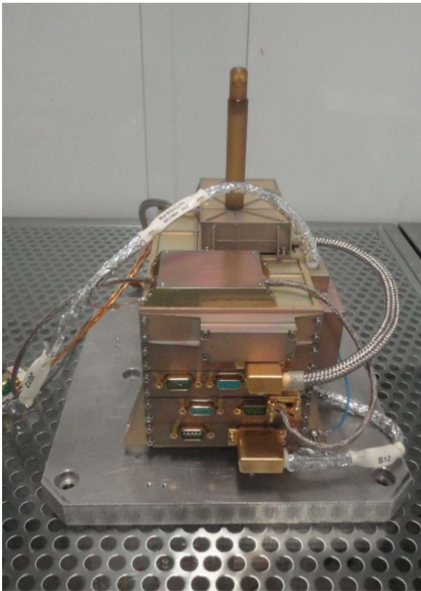
Fig. 5. DREAMS Flight Model of CEU assembly delivered in April 2015.
