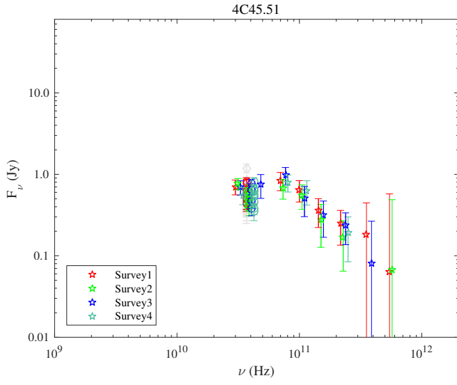
Fig. 1.103. 4C45.51.
