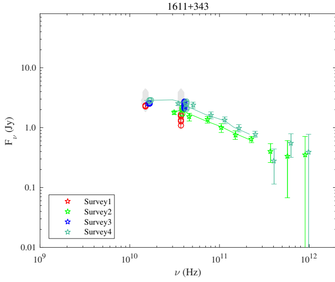
Fig. 1.69. 1611+343.
