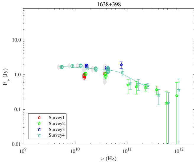
Fig. 1.71. 1638+398.
