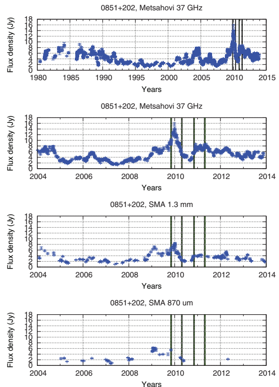
Fig. 7. Flux density curves for 0851+202 at 37 GHz (Metsähovi), 1.3 mm, and 870\mu\text{m} (SMA). See Fig. 6 for details. Some SMA data have been previously published in Agudo et al. (2011) . Some data come from a dedicated programme by Ann Wehrle.
