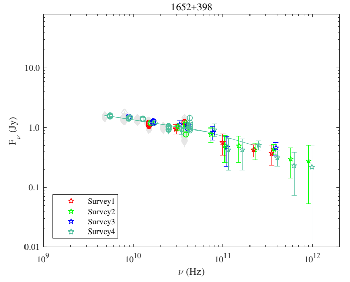
Fig. 1.74. 1652+398.
