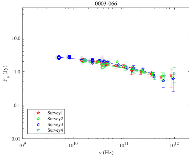
Fig. 1.1. Radio spectrum of 0003–066: coloured stars, Planck data from four Surveys; coloured circles, data simultaneous to the Planck observations; grey circles, historical data and solid lines, broken power-law fits.
