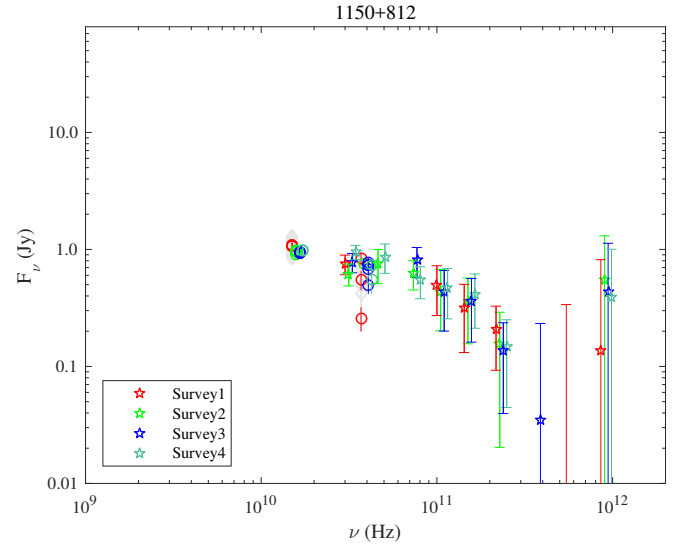
Fig. 1.52. 1150+812.
