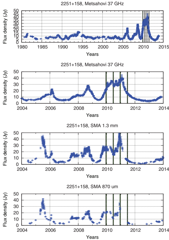
Fig. 10. Flux density curves for 2251+158 at 37 GHz (Metsähovi), 1.3 mm, and 870 \mu m (SMA). See Fig. 6 for details. A large part of the SMA data has been published; see Raiteri et al. (2008, 2011); Villata et al. (2009); Jorstad et al. (2010, 2013); Pacciani et al. (2010); Vercellone et al. (2010, 2011); Ogle et al. (2011); Wehrle et al. (2012). Some data come from a dedicated programme by Ann Wehrle.
