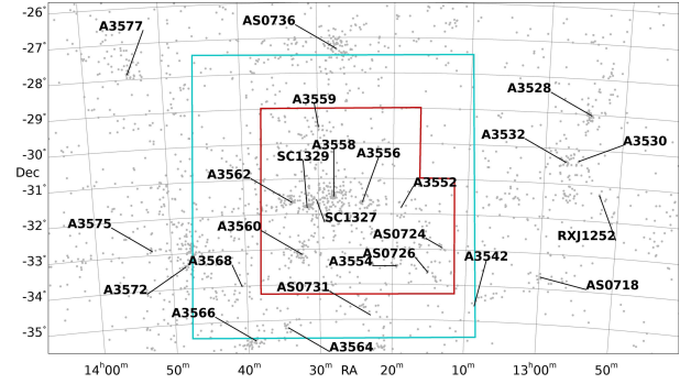
Fig. 1. Location of the clusters and groups in the Shapley Supercluster. The redshift information is from the 6dF Galaxy Survey (6dFGS, Jones et al. 2009 ). The redshift range considered is 0.035 – 0.060 . The cyan lines highlight the area covered by the ASKAP observations (Sect. 3.1), the red lines highlight the coverage of the ESO-VST optical imaging of ShaSS ( Merluzzi et al. 2015 ).
