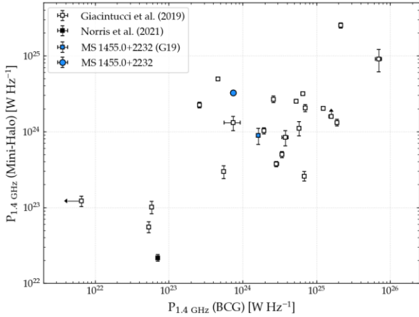
Figure 8. Power scaling plane for mini-haloes, showing how the mini-halo radio power, P_{1.4 \text{ GHz}}(\text{MH}) , scales with BCG radio power, P_{1.4 \text{ GHz}}(\text{BCG}) . Open squares denote known mini-haloes from the sample of Giacintucci et al. (2019), adjusted for differences in assumed cosmology; the black square denotes the mini-halo candidate recently reported by Norris et al. (2021). Blue points indicate the position of MS 1455.0+2232, with the square denoting the measurements from Giacintucci et al. (2019) and the circle indicating our new measurements (note that the uncertainties on our new measurements are not visible at this scale).
