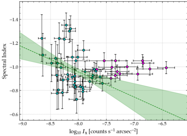
Figure 12. Radio spectral index/X-ray surface brightness correlation for the mini-halo in MS 1455.0+2232. Data points are colourized according to extraction region, as per Fig. 5. Magenta points denote regions inside the boundary of the sloshing spiral, cyan points denote regions exterior to the sloshing spiral. Note the inverted y-axis to facilitate comparison with previous similar studies. Dashed green line shows the best fit to equation (6) for the cyan data points, derived using LINMIX, and the shaded green region shows the 1\sigma uncertainty. The slope is b = 0.21 \pm 0.11 . Magenta points show no correlation.
