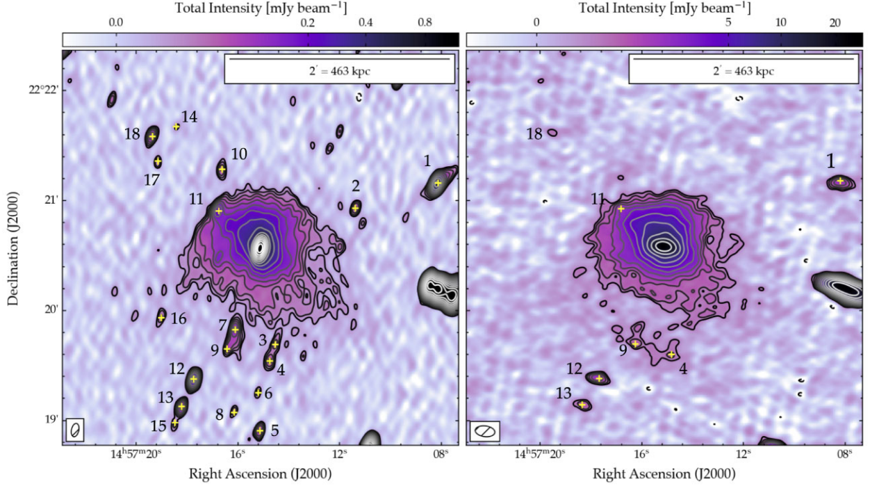
Figure 2. Radio continuum images of MS 1455.0+2232 with MeerKAT at 1283 MHz ( left ) and LOFAR HBA at 145 MHz ( right ) produced using \text{robust} = -0.5 . Image properties (resolution and rms noise) are listed in Table 1; the restoring beam is indicated by the hatched ellipse in the lower-left corner of each subplot. Contours start at 4\sigma and scale by a factor \sqrt{2} . The -4\sigma contour is also shown by dashed lines. Yellow plus signs ( + ) denote sources (other than the BCG) that were modelled and subtracted from each data set; see online supplementary material for flux density measurements and cross-identifications.
