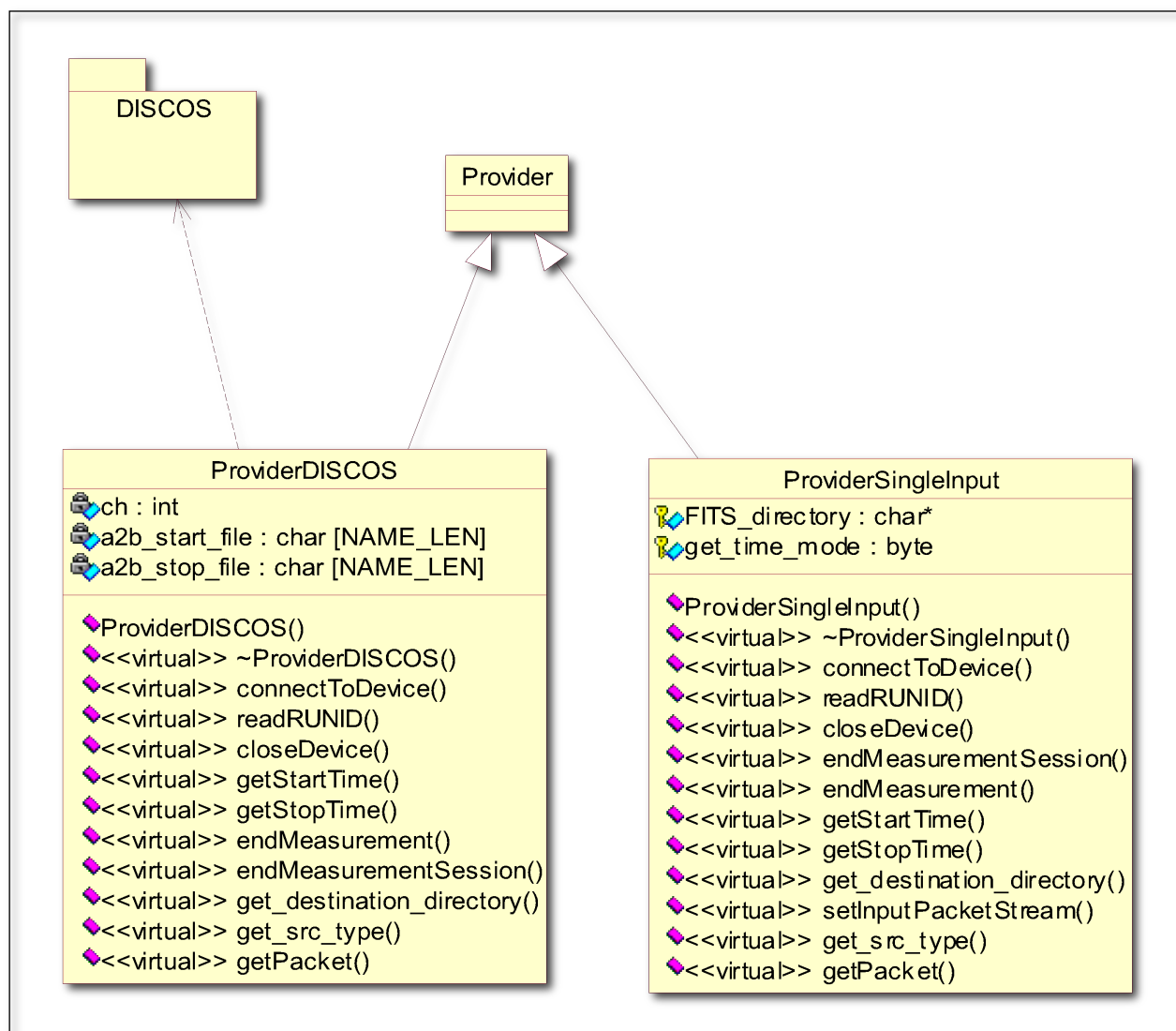
Figure 3: Provider Hierarchy
