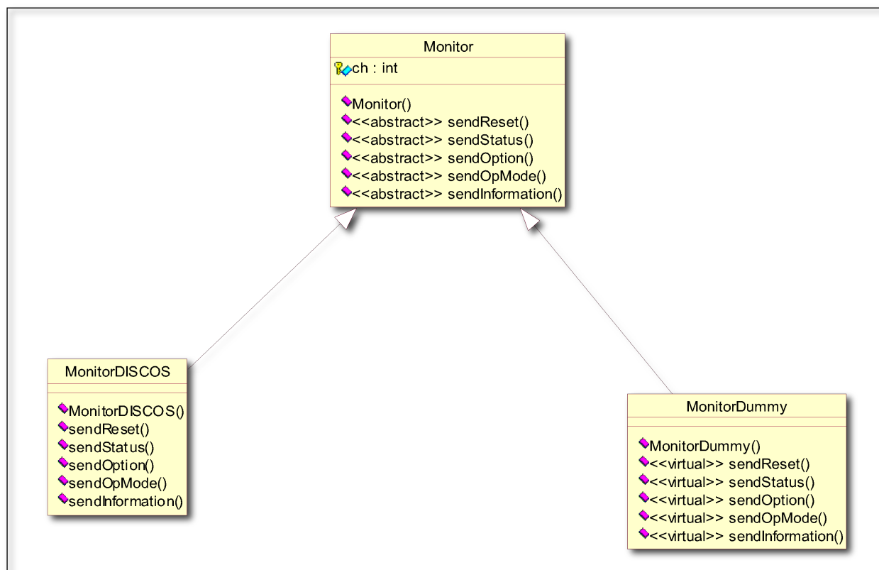
Figure 2: Monitor Hierarchy
