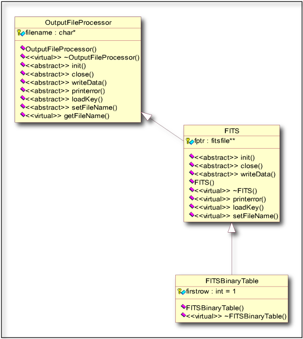
Figure 4: OutputFileProcessor Hierarchy
