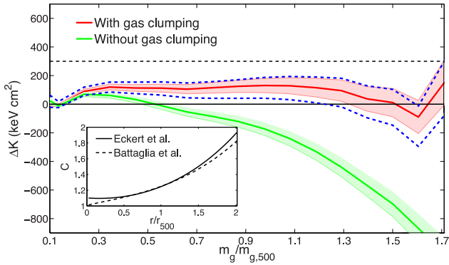
Figure 3. This plot shows the effect on the \Delta K_{\text{feedback}} profile by introducing clumping factor using Eckert et al. (2015) best fit. The shaded region shows 1\sigma error. The region enclosed by two dashed blue lines shows the 1\sigma error band after accounting for clumping errors (15 per cent of the clumping profile). The inset shows comparison of Eckert et al. (2015) and Battaglia et al. (2015) clumping profiles for the average case.
