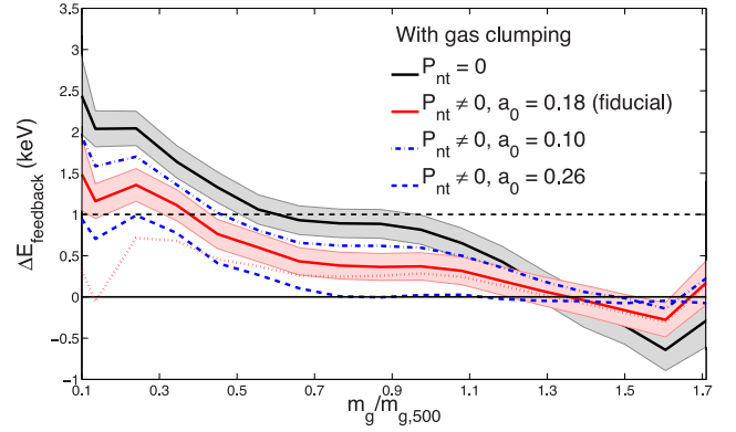
Figure 4. This plot shows the \Delta E_{\text{feedback}} for different normalization a_0 of the non-thermal pressure with larger value of a_0 giving larger non-thermal pressure (see equation 1). We show the 1\sigma error bands for the fiducial case (i.e. a_0 = 0.18 , red band) and the purely thermal case (i.e. a_0 = 0 , grey band). We also show the average profile without adding the energy lost due to cooling (i.e. \Delta E_{\text{ICM}} ) with dotted red line for the fiducial case. For meaningful comparison, we have scaled the x -axis of all the cases with the same m_{g,500} as that of fiducial case.
