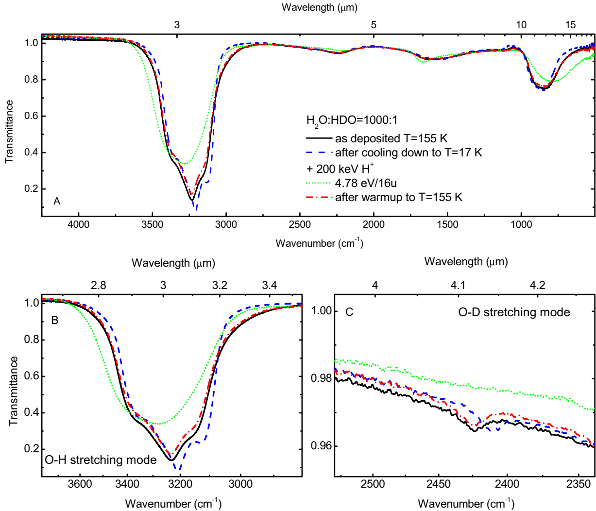
Figure 7. Infrared spectra in transmittance scale acquired during the irradiation experiments of crystalline H 2 O:HDO = 1000:1 with 200 keV H + . Panel A: whole spectra; Panel B: O–H stretching mode band; panel C: O–D stretching mode band.
