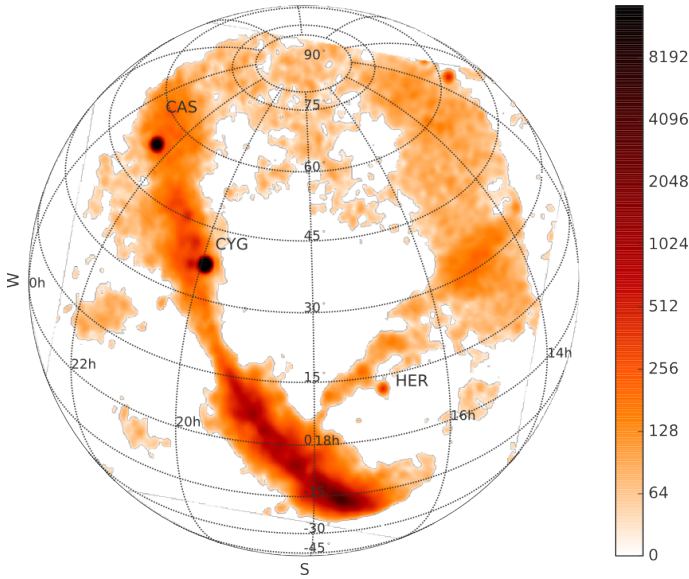
FIG. 8.— Instantaneous all-sky dirty image from LWA-OV using the LEDA512 correlator at night on 2013 August 26 (2.616 MHz centered at 47.004 MHz and 2.13 seconds). The flux scale is normalized to 10^4 Jy for Cyg A. Dominant structures are Cyg A, Cas A, Her A, and the Galactic plane.
