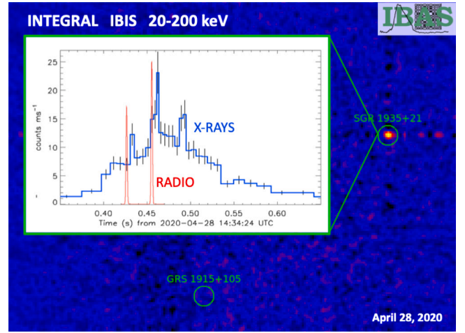
Fig. 3. The localization of the source by the IBAS software and, in the inset, the background subtracted and deadtime corrected light curve derived from IBIS/ISGRI data in the 20–200 keV range. We used an adaptive binning to ensure at least 40 counts per time bin. All the times are in the geocentric frame and referred to t_0 = 14:34:24 UTC of April 28, 2020. The red line (adapted from Fig. 1 of CHIME/FRB Collaboration et al., 2020) marks the position of the radio pulses, represented with two Gaussian curves centered at 0.42648 s and 0.45545 s.
