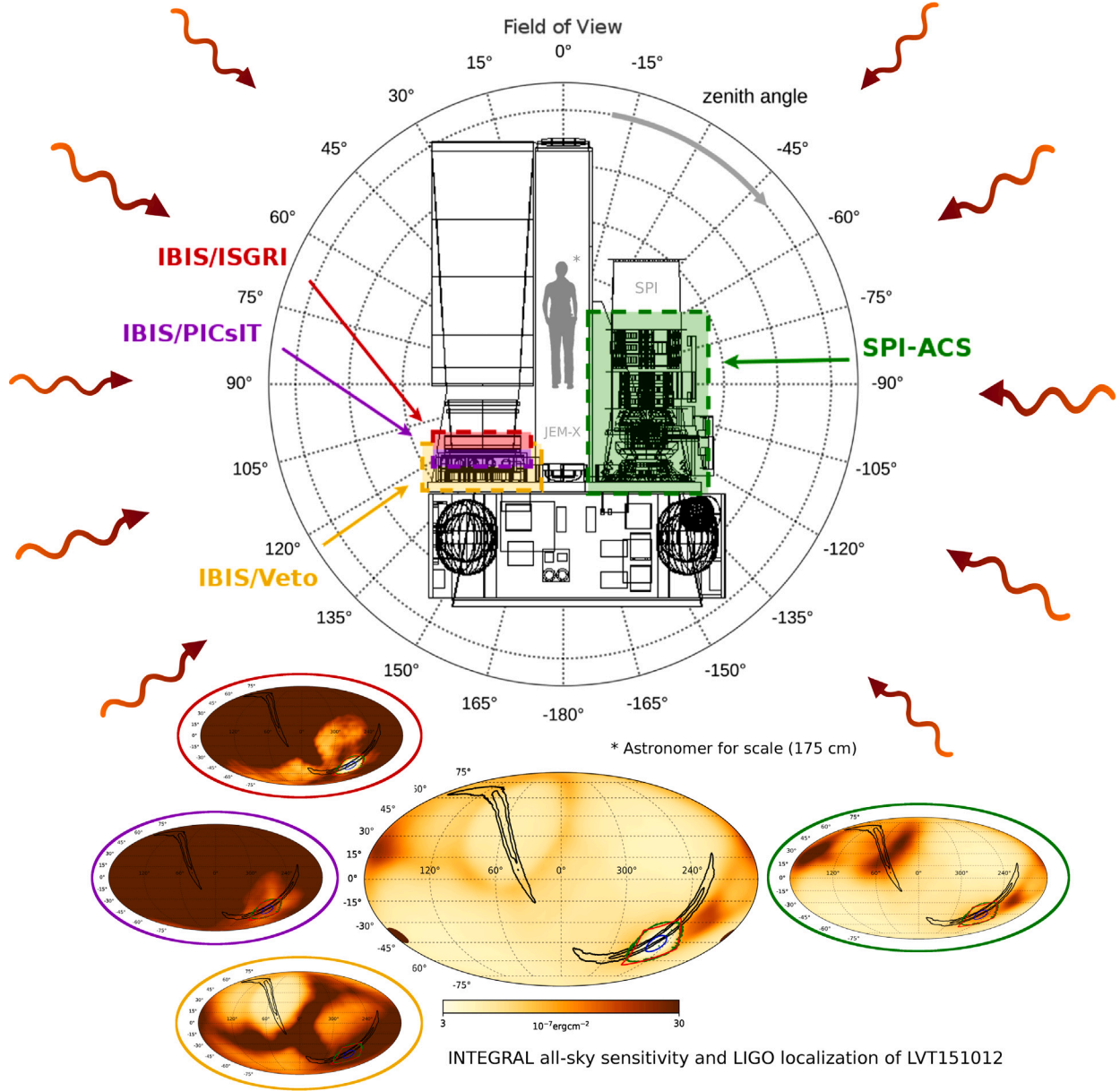
Fig. 1. INTEGRAL's unique payload is comprised of a set of large and heavy detectors with sensitivity optimized in the field of view for SPI (gray), IBIS/ISGRI (red) and IBIS/PICsIT (violet), but extended marginally to the whole sky. Particle and radiation shields of the spectrometer (SPI-ACS in green) and of the imager (IBIS-Veto in yellow) are truly sensitive to the full sky at a level competitive with currently flying gamma-ray burst monitors. In the bottom, we show sensitivity maps of SPI-ACS, IBIS/Veto, IBIS/PICsIT, and IBIS/ISGRI for the detection of an 8 s soft GRB event at 3\sigma confidence level whose spectral energy distribution is described by a Comptonized model with parameters \alpha = -1 and E_p = 300 keV). We represent with black contours the most accurate localization of the GW event (at 50% and 90% confidence levels). Red, green, and blue contours indicate the sky regions within which the respective sensitivity of ISGRI, SPI, and JEM-X is not degrading more than a factor of 20 compared to the on-axis value. Observation of the complete, extended, localization region could only be achieved by combining the complementary contributions of both the INTEGRAL high-energy detectors and their active shields. This allowed the INTEGRAL team to derive the most stringent upper limit in a truly all-sky observation, constraining the ratio of energy released in gamma-rays to the gravitational wave energy to less than 4.4 \times 10^{-5} .
