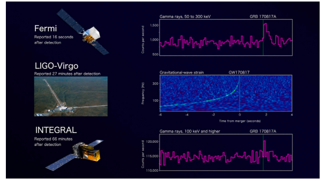
Fig. 2. The joint, multi-messenger detection of GW170817 and GRB170817A. Top: The summed Fermi/GBM lightcurve for sodium iodide (NaI) detectors 1, 2, and 5 for GRB170817A between 50 and 300 keV, matching the 100 ms time bins of SPI-ACS data shown at the bottom. Middle: The time–frequency map of GW170817 was obtained by coherently combining LIGO-Hanford and LIGO-Livingston data. Bottom: The SPI-ACS lightcurve with the energy range starting approximately at 100 keV and with a high energy limit of at least 80 MeV. All times here are referred to the GW170817 trigger time.
