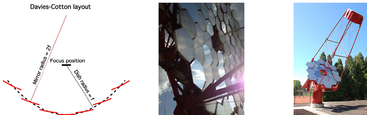
Figure 4 Left: Scheme of the Davies-Cotton optical design. Mirrors with radius of curvature 2f are arranged on a mechanical structure with radius f . Center: the MST prototype with the mirrors manufactured by the authors. Right: the SST-1M prototype with dummies.
